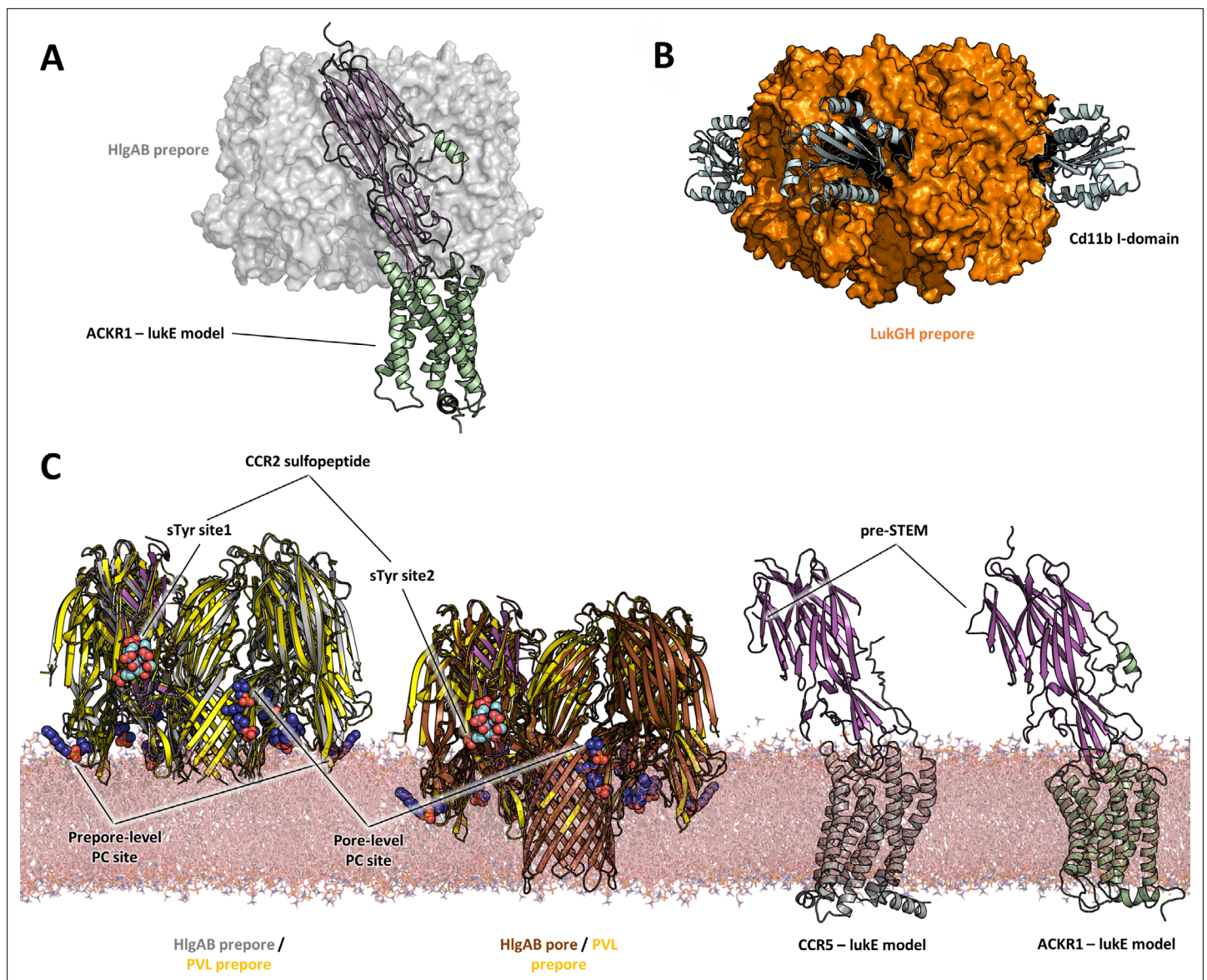
Figure 10. Comparisons of Luke-CCR2 peptide x-ray structure, ACKR1-LukeE and CCR5-LukeE models with existing x-ray structures. (A) Structural alignment of LukeE from the ACKR1-LukeE model with the HlgAB prepore structure (PDB ID 4P1Y), illustrating that the N-terminal region of ACKR1 binds to a surface located on the outer part of the prepore. The HlgAB prepore is shown as a semitransparent surface and the ACKR1-LukeE model as cartoon. (B) X-ray structure of LukGH bound to human CD11b I-domain. The LukGH prepore is shown as a semitransparent surface and the CD11b I-domain as cartoon. (C) The HlgAB pore and prepore structures (PDB IDs 3B07 and 4P1Y) are shown in their membrane context using a POPC bilayer extracted from MDS simulations. On the left, the HlgAB pore and prepore structures are superimposed to the PVL prepore (PDB ID 6U3Y) bound with fos-choline-14 (shown as blue spheres). One of the lukF-PV/HlgB protomer is omitted for clarity. The structural alignment highlights the presence of lipid headgroup binding sites on lukF-PV that correspond to different membrane insertion depths, which we interpreted as pore and prepore membrane levels. The Luke-CCR2 peptide structure is also superimposed onto the pore and prepore structures to indicate the location of the bound sulfotyrosines (shown as cyan spheres). In the case of a fully formed pore, sTyr sulfate at site 2 is located at the same level as the PC headgroups. On the right, the ACKR1-LukeE and CCR5-LukeE models are shown in their membrane context, and oriented to visualize the acute angle between LukeE and the membrane.
