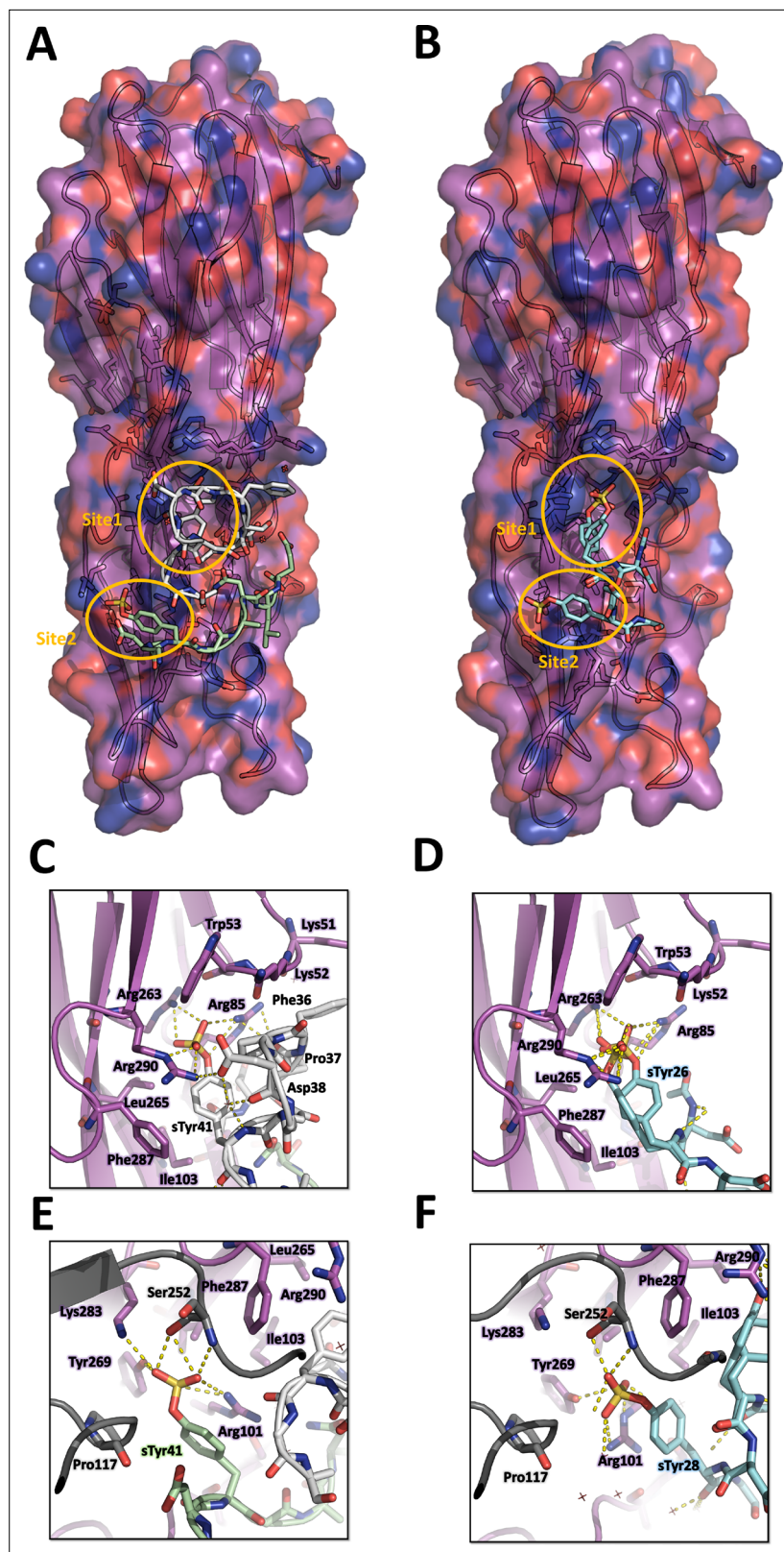
Figure 4. Crystal structures of LukE in complex with ACKR1 peptide ^{34}\text{DSFPDGDsYGANLE}^{46} and CCR2 peptide ^{25}\text{DsYDsYG}^{29} . (A) Overview of the asymmetric unit of the ACKR1 peptide-soaked crystal. Protein is shown in cartoon representation and colored in magenta. The two copies of the peptide with their respective sulfotyrosine residue bound to site 1 and 2 are shown in white and green cartoon and sticks representation. Surrounding protein Figure 4 continued on next page
