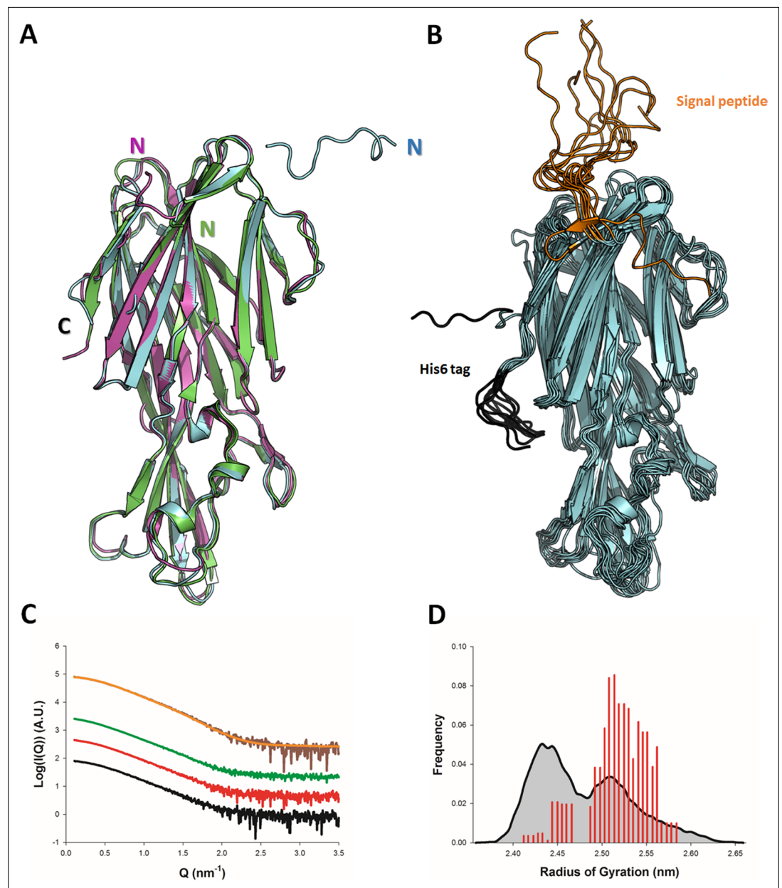
Figure 1. Solution and crystallographic structures of leukotoxin LukE. (A) The crystal structures of LukE in P2 1 ,2 1 ,2 1 (Apo 1, green) and I4 (Apo 2, cyan) space groups are shown in cartoon representation and overlaid onto the previously published crystal structure of LukE (magenta), also in I4 space group (PDB code 3ROH). (B) Optimized ensemble of 10 models corresponding to the fitted SAXS profile in C. The N-terminal extension belonging to the signal peptide and the C-terminal polyhistidine tag are shown in orange and black, respectively. The CAP, RIM, and STEM domains are colored in cyan, deep blue and light blue, respectively. Other regions of interest are also indicated such as the D-region, and divergent loops 1–4. (C) Small angle x-ray scattering (SAXS) profiles of LukE measured at 1, 2, and 4 mg/ml are shown as black, red and green lines, respectively. The merged SAXS curve is shown as a brown line with the fitting curve obtained using the ensemble optimization method (EOM) in orange. (D) Radius of gyration distributions for the initial pool ensemble (gray area and black line) and for the optimized ensembles (red bars) obtained using the merged SAXS curve.
