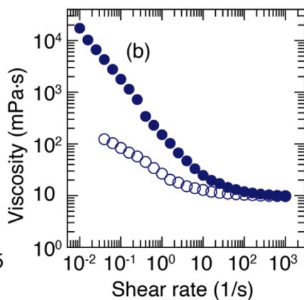
Fig. 6. Time-course change in (a) Storage (filled circles in dark blue) and loss modulus (open circles in dark blue) of GA solution filled with vegetable oil. Storage and loss modulus just after the complete shearing with flow sweep test are shown with filled (storage) and open (loss) circles in light-blue; (b) Viscosity flow curve of GA solution 22 h after the filling (filled circles in dark blue) and just after the filling (open circles). The measurement was performed by a flow sweep test, wherein the shear rate was increased by steps from 0.01 to 1000 s^{-1} .
