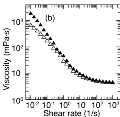
Fig. 4. (a) Time-course change in Storage (filled triangle) and loss (open triangle) modulus. Storage and loss modulus just after the complete shearing with flow sweep test are shown with filled (storage) and open (loss) circles in violet; (b) Viscosity flow curve of GA solution 14 h after the filling (filled triangles in black) and just after the filling (open triangles, same plots as in Fig. 2). The measurement was performed by a flow sweep test, wherein the shear rate was increased by steps from 0.01 to 1000 s^{-1} .
