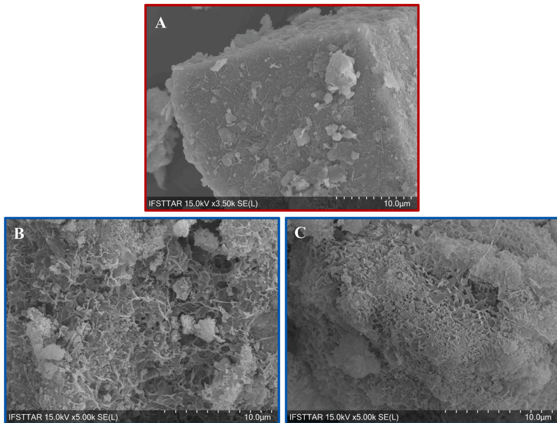
Fig. 5. SEM images of the marlstone calcined at 800 °C (A) and hydrated for 28 days (B and C).
