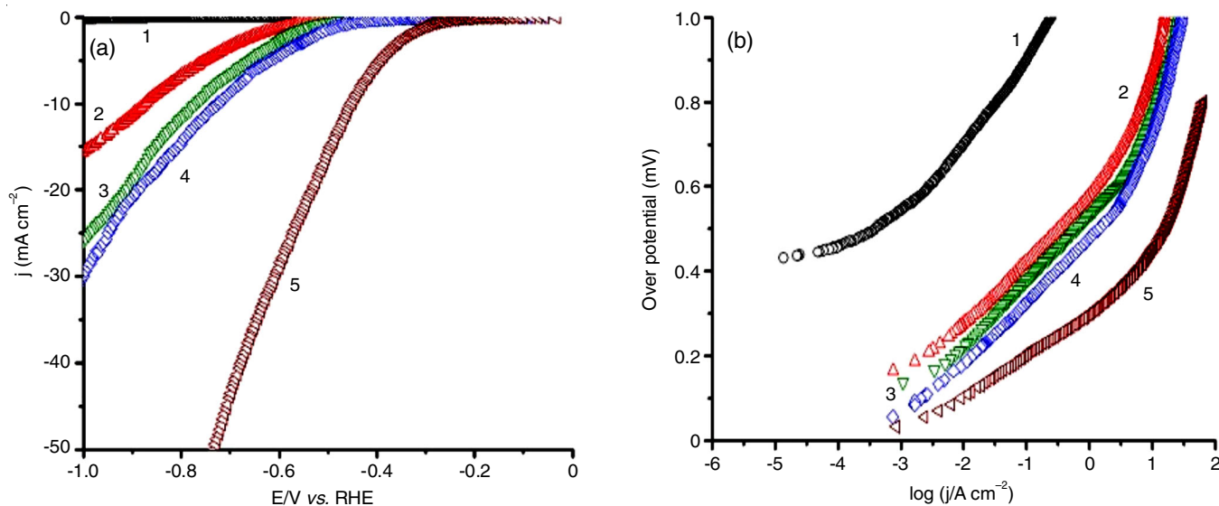
Fig. 3. (a) LSV measurements constructed for the studied \text{Zn2} of various loading densities in a comparison with bare GC and Pt/C. Measurements were carried out in 0.1 M KOH aqueous solution at a scan rate of 5.0 \text{ mV s}^{-1} at room temperature. (b) Tafel plots derived from the LSV data (a). (1) bare GC; (2) GC- \text{Zn2} ( 0.1 \text{ mg cm}^{-2} ); (3) GC- \text{Zn2} ( 0.3 \text{ mg cm}^{-2} ); (4) GC- \text{Zn2} ( 0.5 \text{ mg cm}^{-2} ); (5) Pt/C
