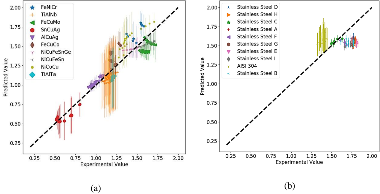
Figure 7 ML-GPR model prediction vs experimental values of ST [ N.m^{-1} ] for several higher order system including several stainless steels grades (stainless steels A to I [40], AISI 304 [37]), when the model is learnt solely from pure metals and binary alloys
