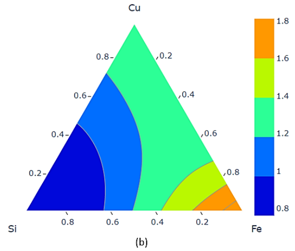
Figure 6 ML-GPR Prediction of Surface Tension [ N.m^{-1} ] for a) Cr-Co-Ni at 1873K and b) Cu-Si-Fe at 1773K
