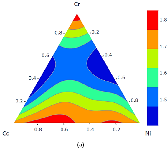
Figure 6 ML-GPR Prediction of Surface Tension [ N.m^{-1} ] for a) Cr-Co-Ni at 1873K and b) Cu-Si-Fe at 1773K
