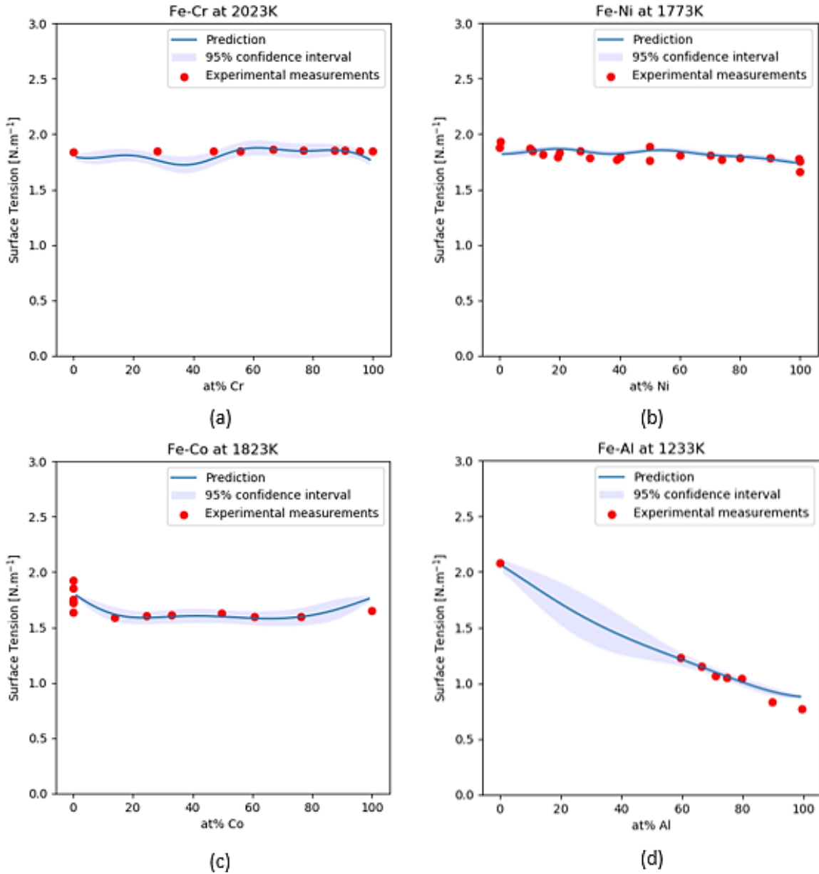
Figure 3 Surface tension prediction for a) Fe-Cr at 2023 K, b) Fe-Ni at 1773 K, c) Fe-Co at 1823 K and d) Fe-Al at 1233 K
