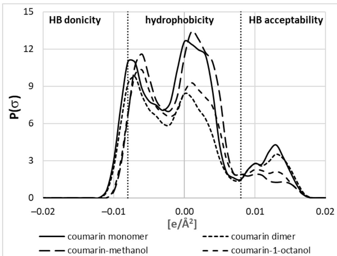
Figure 6. Exemplary \sigma -profile plots characterizing the coumarin monomer not involved in direct contacts, the dimer in stacked conformation, and hydrogen-bonded heteromolecular pairs with methanol and 1-octanol. The hydrophobicity region was defined as the charge density range between -0.08 and +0.08 \text{ e} \cdot \text{\AA}^{-2} .
