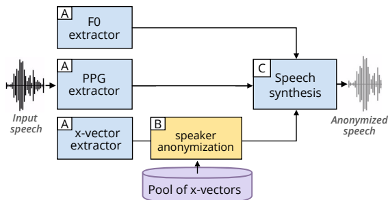
Figure 1: The speaker anonymization pipeline.
