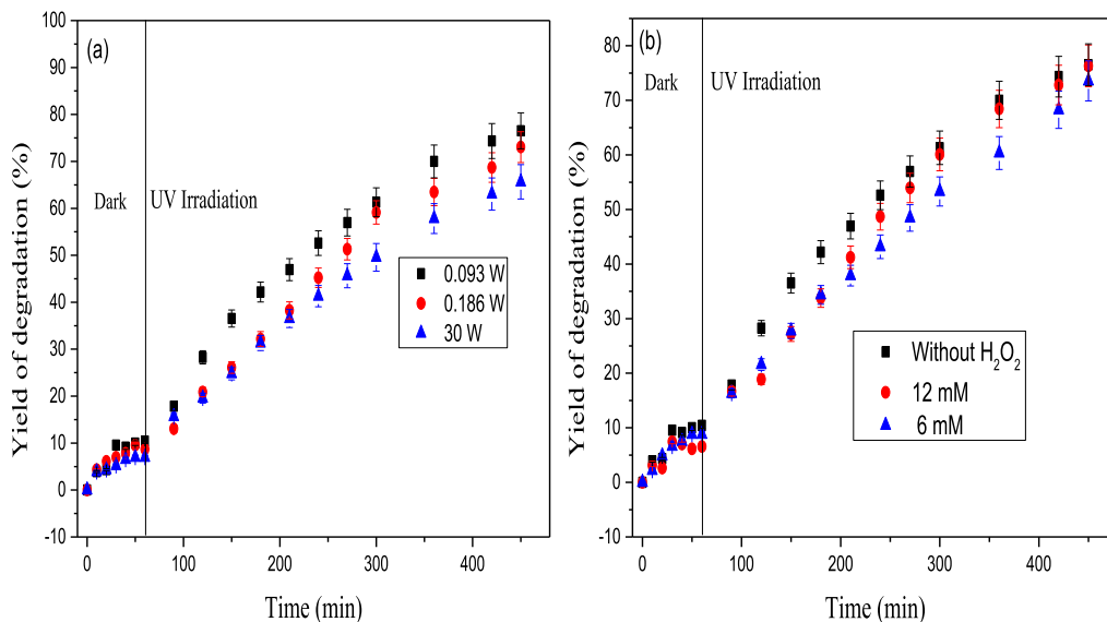
Figure 7. (a) Evolution of the degradation rate during the photocatalytic process: effect of light intensity ( \text{pH}_{30\text{ W}} = 7.19 , \text{pH}_{0.186\text{ W}} = 6.37 , \text{pH}_{9.2 \times 10^{-2}\text{ W}} = 7.11 , C_0 = 5_{\text{RBBR}}/5_{\text{DR227}} \text{ mg}\cdot\text{L}^{-1} ), (b) evolution of the degradation rate during the photocatalytic process: effect of the addition of \text{H}_2\text{O}_2 ( \text{pH}_{6\text{ mM}} = 6.73 , \text{pH}_{12\text{ mM}} = 7.01 , C_0 = 5_{\text{RB19}}/5_{\text{DR227}} \text{ mg}\cdot\text{L}^{-1} , P = 0.093\text{ W} ).
