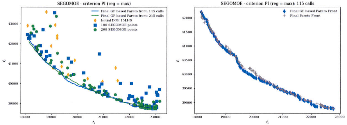
(a) Approximate Pareto fronts obtained with SEGOMOE - PI (reg = max) criterion: 115 and 215 calls (b) Approximate Pareto front (SEGOMOE - PI (reg = max), 115 calls) and the recomputed one with FAST-OAD.
