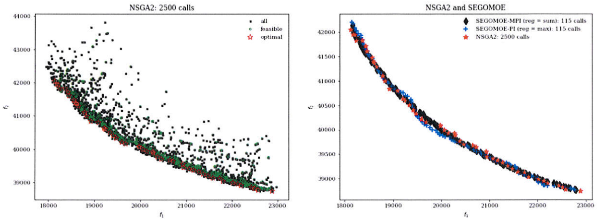
(a) Admissible points, dominated points and Pareto front using NSGA-II. A total of 2500 points is represented. (b) Comparison of Pareto fronts obtained with SEGOMOE (115 calls) and NSGA-II (2500 calls)
