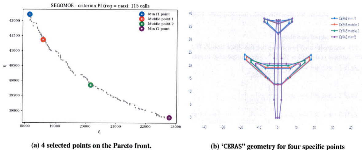
Fig. 10 "CERAS" geometry configurations for four selected points on the Pareto front.
