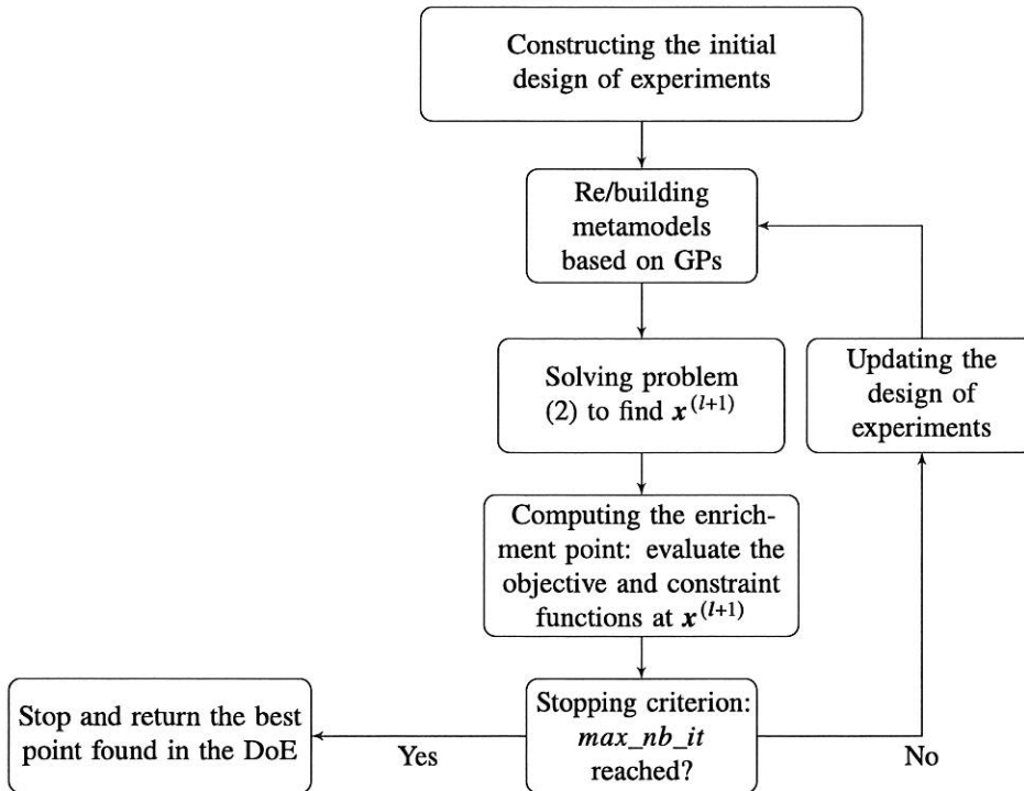
Fig. 1 The summary of SEGOMOE algorithm steps.
