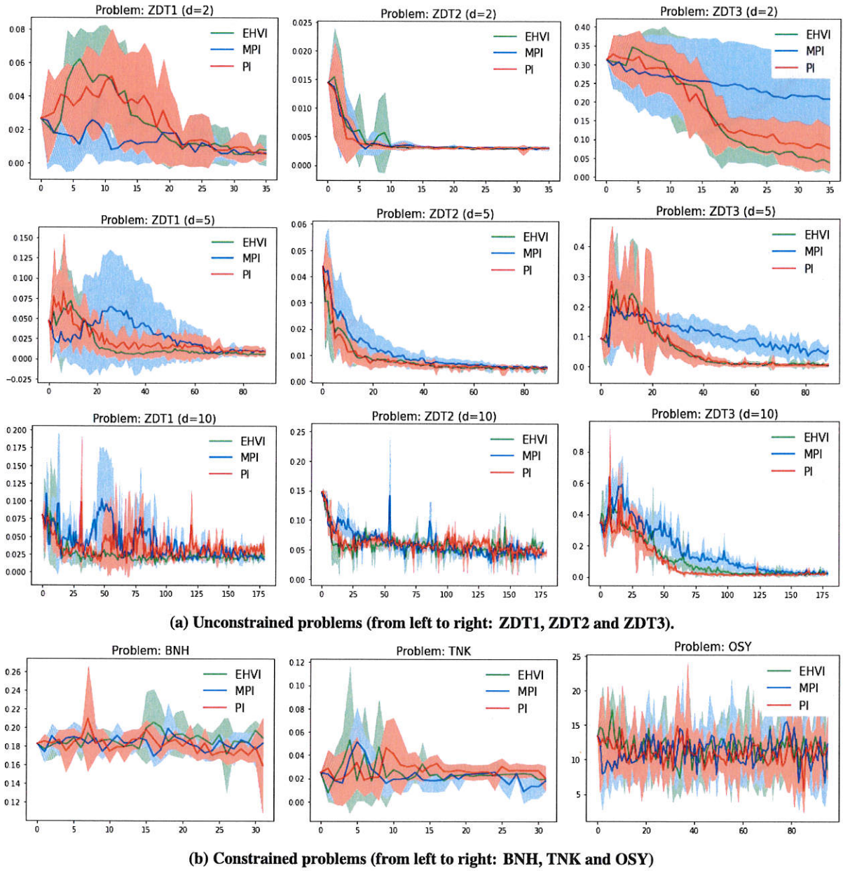
Fig. 2 Obtained convergence plots (i.e., IGD^+ values across iterations): a comparison of the acquisition functions EHVI , PI and MPI within SEGOMOE using IGD^+ .
