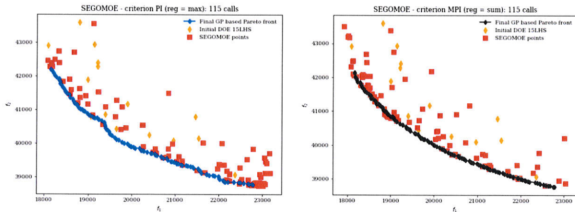
(a) Approximate Pareto front obtained with SEGOMOE - PI (reg = max) criterion (b) Approximate Pareto front obtained with SEGOMOE - MPI (reg = sum) criterion
