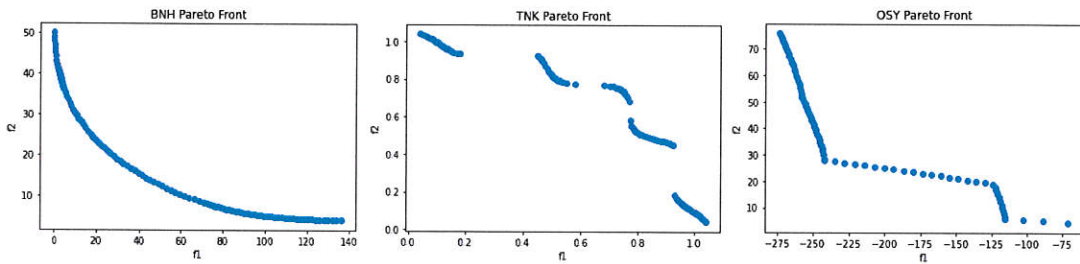
Fig. 13 The optimal Pareto fronts of the tested constrained multi-objective problems: BNH, TNK and OSY.
