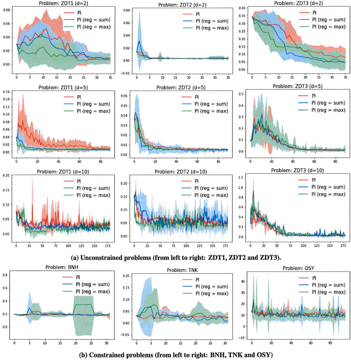
Fig. 4 Obtained convergence plots (i.e., IGD^+ values across iterations): regularization effect on the PI acquisition function within SEGOMOE.
