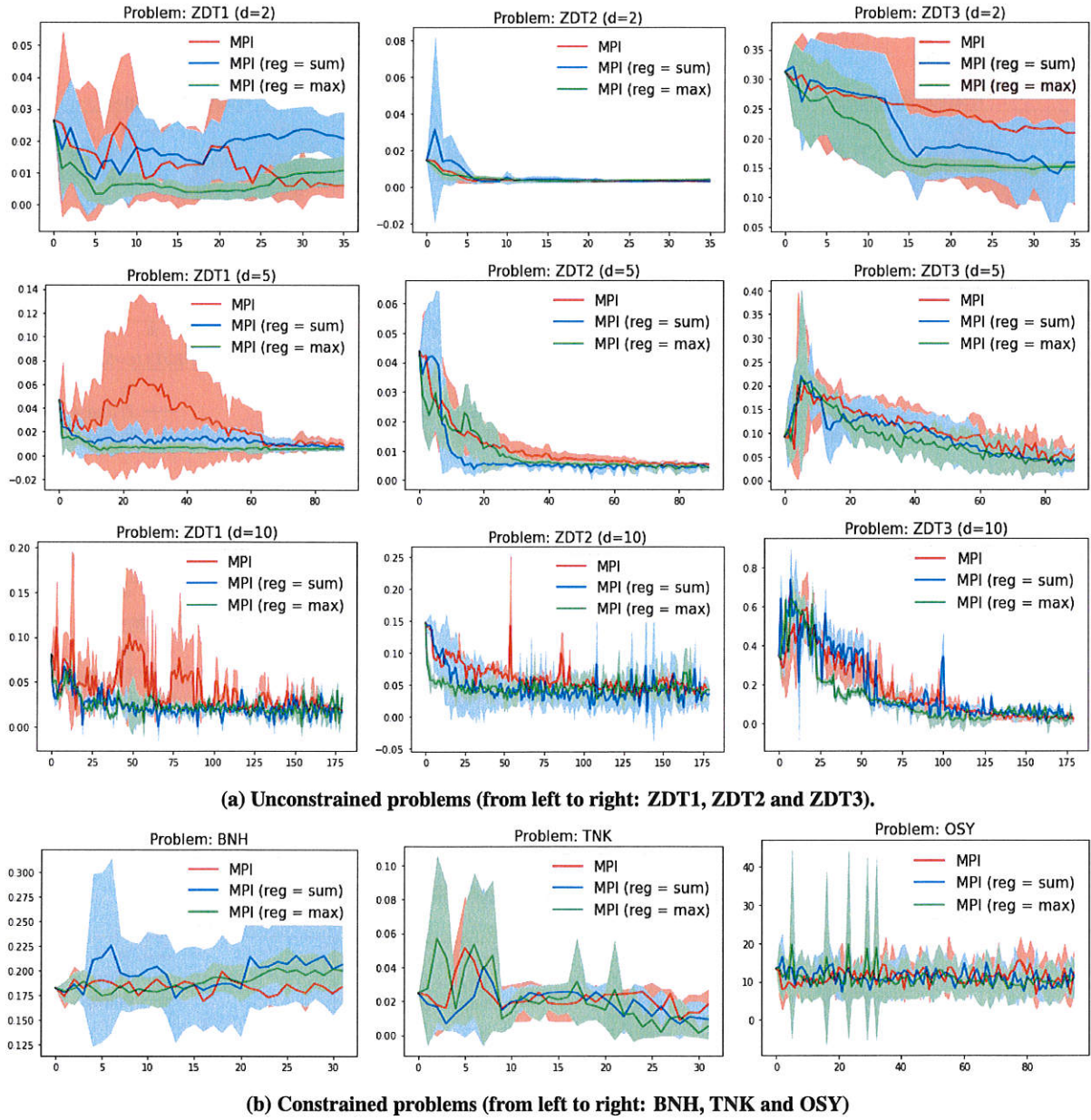
Fig. 5 Obtained convergence plots (i.e., IGD^+ values across iterations): Regularization effect on the MPI acquisition function within SEGOMOE.
