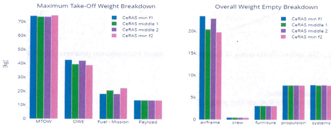
Fig. 11 Mass breakdown: Maximum TakeOff Weight and Overall Weight Empty for the four selected "CERAS" different configurations.
