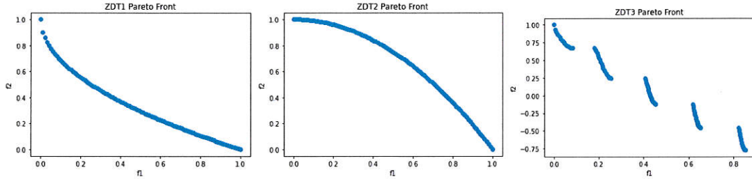
Fig. 12 The optimal Pareto fronts of the tested unconstrained multi-objective problems: ZDT1, ZDT2 and ZDT3.
