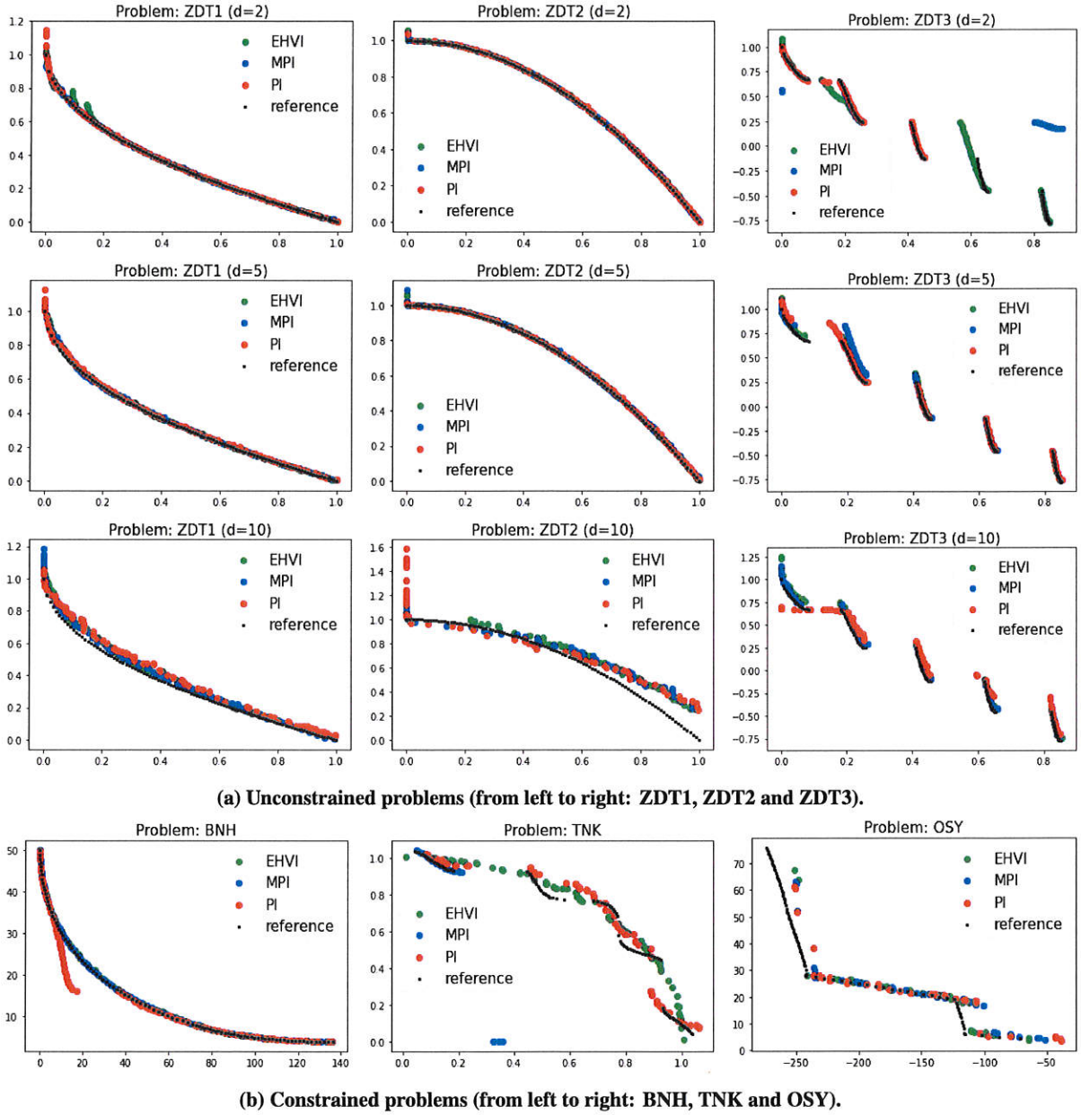
Fig. 3 A comparison of the obtained Pareto fronts obtained using 20d points on the
