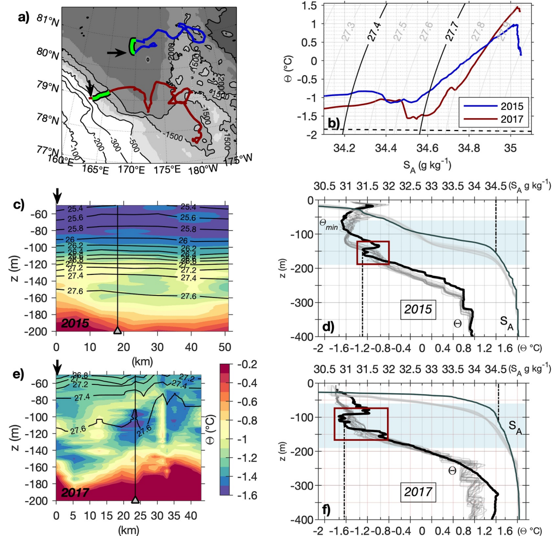
Figure 10. (a) Trajectories of IAOOS15 (blue) and IAOOS25 (red). Cold lenses were found in the green subsections. (b) Temperature-salinity curve in the cold lens for IAOOS15 (blue) and IAOOS25 (dark red). (c) IAOOS15 (September 2015) temperature along the green subsections, and (d) temperature (black thick lines) and salinity (dark gray thick lines) profiles in the cold lens area. The temperature minimum corresponding to the cold core of the lens is highlighted by a red box. (e and f) Same for IAOOS25 (November 2017). The beginning of the section is indicated by an arrow in (a), (c), and (e) and the position of the cold lens is indicated by thick vertical black lines. Light gray profiles in (d) and (f) are outside the cold lens area (15 profiles preceding the green subsection in time) and vertical dotted lines indicate temperature and salinity in the cold lens. The blue shade corresponds to the depths shown in sections (c) and (e). Corresponding synoptic horizontal PSY4 fields are shown in Figure S4 in Supporting Information S1.
