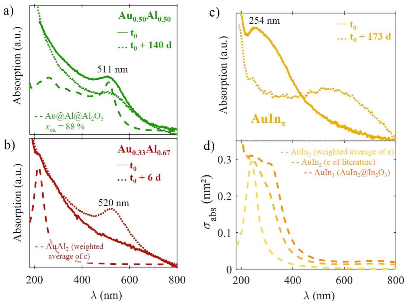
Fig. 5: Optical responses of \text{Au}_{0.50}\text{Al}_{0.50} (a), \text{Au}_{0.33}\text{Al}_{0.67} (b), \text{AuIn}_x ( 2 < x < 3 ) (c and d). (solid line): experimental absorption spectra of \text{Au}_{0.33}\text{Al}_{0.67} , \text{Au}_{0.50}\text{Al}_{0.50} and \text{AuIn}_x ( 2 < x < 3 ) silica-embedded BNPs at time t_0 (a few tens of minutes after venting). (dotted line): experimental spectra after n days upon exposure to air (time t_0 + n d). (dashed lines): simulated absorption cross-sections for various configurations - (a): \text{Au@Al@Al}_2\text{O}_3 spherical structure with a volume oxidation rate of 88%. (b): homogeneous alloyed sphere \text{AuAl}_2 using the weighted average dielectric function of Au and Al. (d): respectively from the yellow to the orange curve: alloyed phase \text{AuIn}_2 using the weighted average dielectric function of Au and In; ordered homogeneous alloyed phase \text{AuIn}_2 whose dielectric function is taken from the literature 21 ; spherical core-shell structure of average composition \text{Au}_{0.25}\text{In}_{0.75} , with a core of \text{AuIn}_2 (dielectric function taken from 21 ), and a shell of indium oxide.
