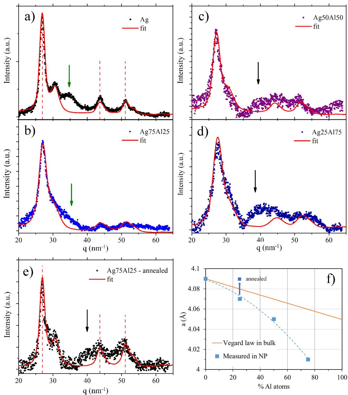
Fig. 2 (a-d) Four GIWAXS spectra of silver-based pure Ag, Ag 0.75 Al 0.25 , Ag 0.50 Al 0.50 , Ag 0.25 Al 0.75 BNPs with the superimposition of simulations of a model NP spectrum (fit from size distribution); (e) GIWAXS spectrum of annealed Ag 0.75 Al 0.25 BNPs (sample b) at 350°C; (f) Crystalline lattice parameters a obtained from average BNP interatomic distance extracted from simulated spectrum, reported versus the average % of Al atoms. The black arrows in the spectra in the range 40-50 nm -1 correspond to additional contributions that may be attributed to aluminium oxide. The green arrows correspond to signal which comes from the variation in the substrate-carbon contribution from a sample to another.
