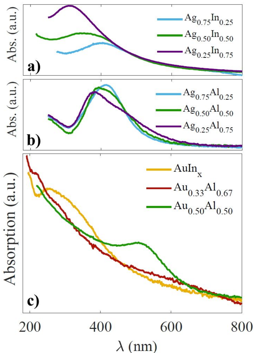
Fig. 4: (a): experimental absorption spectra of non-size-selected \text{Ag}_x\text{In}_{1-x} silica-embedded BNPs. The average diameter is around 4 nm with a size dispersion of 80% of their diameter. (b): experimental absorption spectra of size-selected \text{Ag}_x\text{Al}_{1-x} silica-embedded BNPs. Their mean diameters are \langle \phi \rangle = 4.3 nm, 4.1 nm and 3.8 nm for \text{Ag}_{0.25}\text{Al}_{0.75} , \text{Ag}_{0.50}\text{Al}_{0.50} and \text{Ag}_{0.75}\text{Al}_{0.25} , respectively. (c): experimental absorption spectra of size-selected \text{Au}_{0.33}\text{Al}_{0.67} , \text{Au}_{0.50}\text{Al}_{0.50} \text{AuIn}_x ( 2 < x < 3 ) silica-embedded BNPs. Their mean diameters are \langle \phi \rangle = 5.5 nm, 4.1 nm and 4.2 nm for \text{Au}_{0.33}\text{Al}_{0.67} , \text{Au}_{0.50}\text{Al}_{0.50} and \text{AuIn}_x ( 2 < x < 3 ), respectively.
