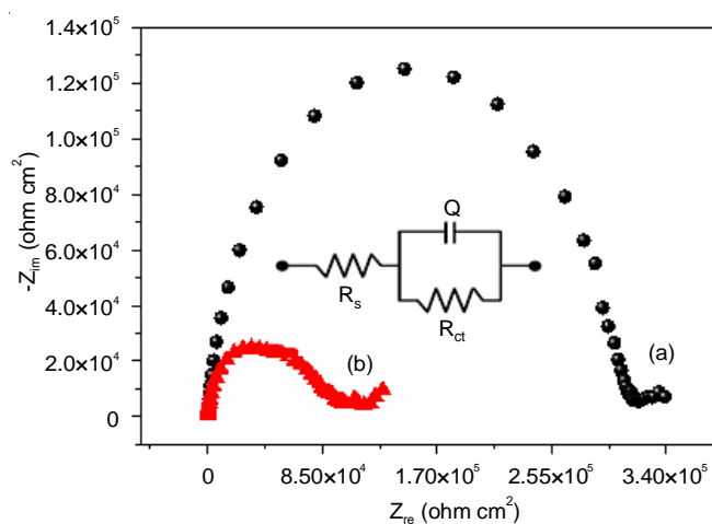
Fig. 2. Nyquist plots of CPE (a) and CP-KT xylyl modified electrode (b) in a solution containing 5 mM [\text{Fe}(\text{CN})_6]^{3-/4-} and 1 M KCl, (inset equivalent circuit for system). Inset: R_s (the solution/electrolyte resistance), Q a constant phase element corresponding to the double layer capacitance and R_{ct} is the charge transfer resistance associated with the oxidation of low valence mediator pieces
