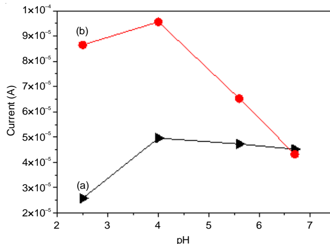
Fig. 3. Dependence of peak current height on pH for (a) 1 \times 10^{-3} \text{ M} \text{Cd}^{2+} and \text{Pb}^{2+} ions and a CPE-KT xylyl modified electrode
