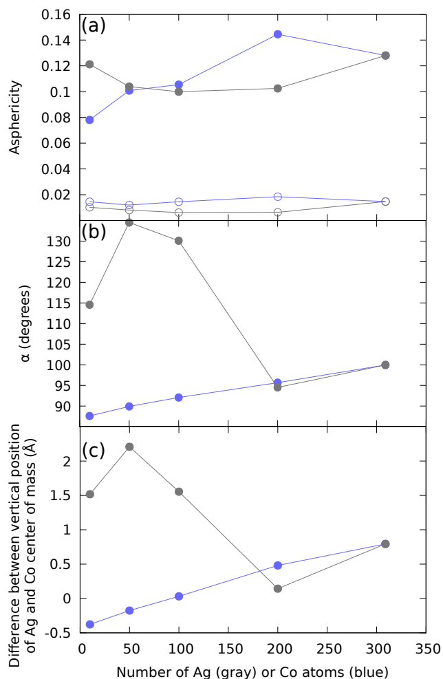
Fig. 2 Particle geometry and orientation at thermodynamic equilibrium at 300K for free particles (open circles) and particles in contact with an amorphous carbon substrate (full circles) as a function of chemical composition. Particles always contain 309 atoms of one metal (Ag or Co) and a variable number of atoms of the respective other species, represented on the x -axis. (a) Particle asphericity. (b) Particle orientation (same definition as Fig. 1-c). (c) Relative vertical position of the Co and Ag center of mass.
