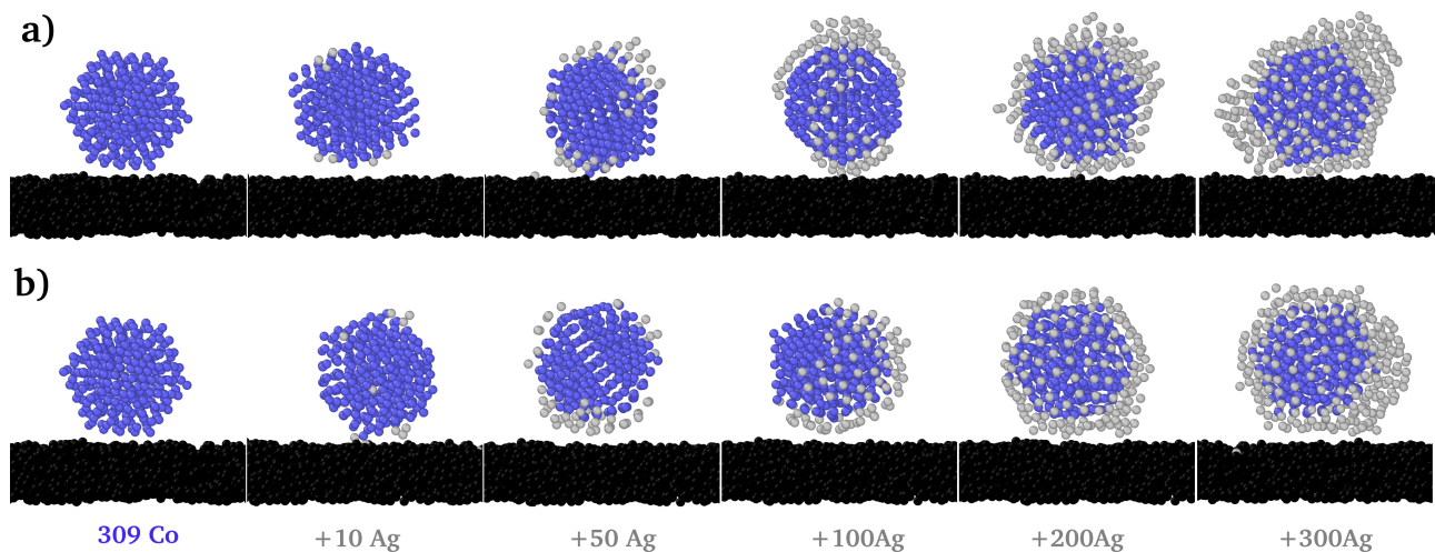
Fig. 4 Snapshots of the growth of Ag on an initial Co nanoparticle( Ih_{Co309} ) supported on an amorphous carbon substrate. The snapshots are taken at different stages of growth until 50% Ag atom content. Co and Ag atoms are represented as blue and gray spheres, respectively. (a) Sequence at 300 K, (b) Sequence at 600 K
