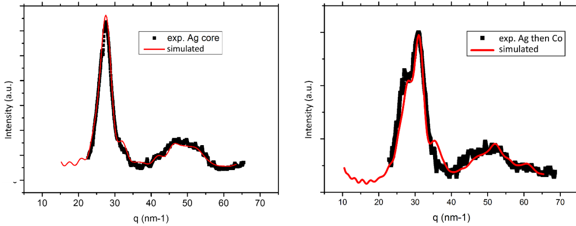
Figure S2 : GIWAXS spectra : (left) Initial Ag particle, and (right) Ag particle after Co deposition (until the AgCo 2 composition), associated respectively with the simulated spectrum (red line) coming (left) from icosahedral distribution of Ag models centered on 309 atoms in size, and (right) from a Co-core/Ag-shell model of Ag 309 Co 600 atoms.
