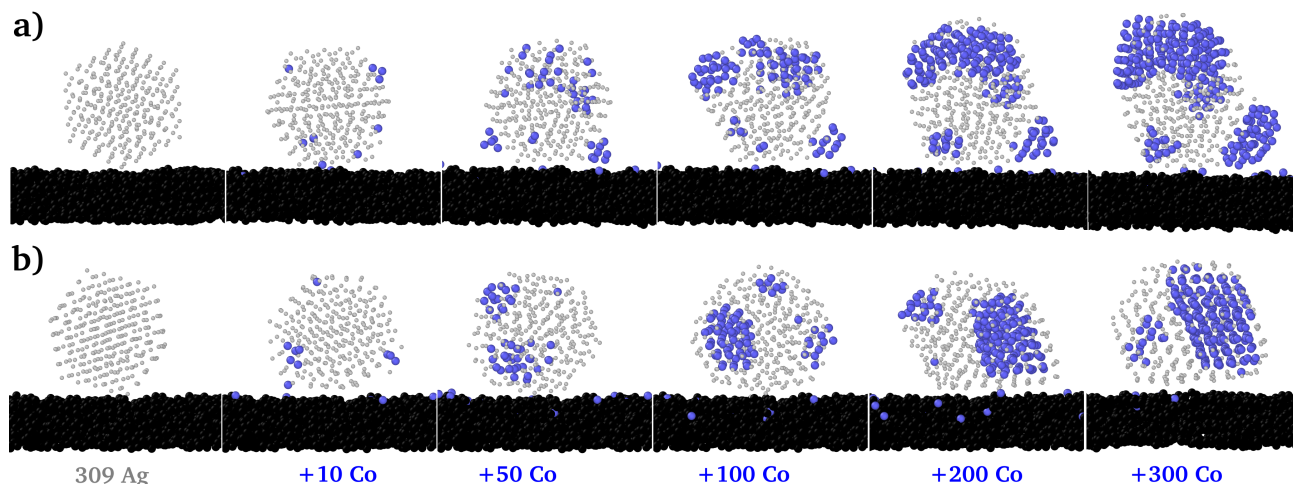
Fig. 6 Snapshots of the growth of Co on an initial Ag nanoparticle ( Ih_{Ag309} ) supported on an amorphous carbon substrate. The snapshots are taken at different stages of growth of up to 50% Ag content. Co and Ag atoms are represented as blue and gray spheres, respectively. (a) Sequence at 300 K, (b) Sequence at 600 K
