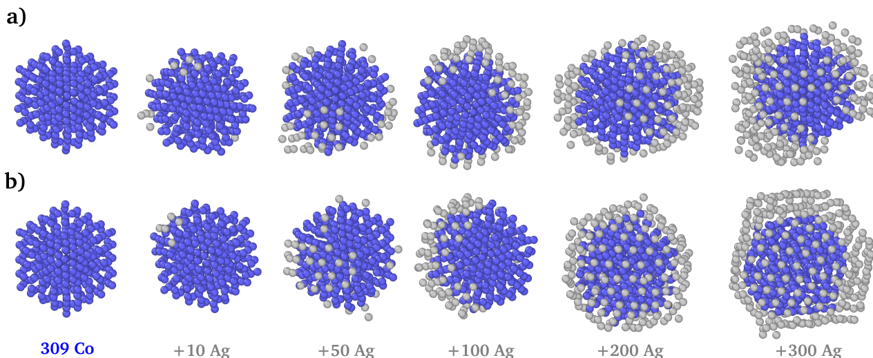
Fig. 3 Snapshots of the growth of Ag on an initial free Co nanoparticle ( Ih_{Co309} ) at 300K (a) and 600K (b). The snapshots are taken at different stages of growth until 50% Ag content. Co and Ag atoms are represented as blue and gray spheres, respectively.
