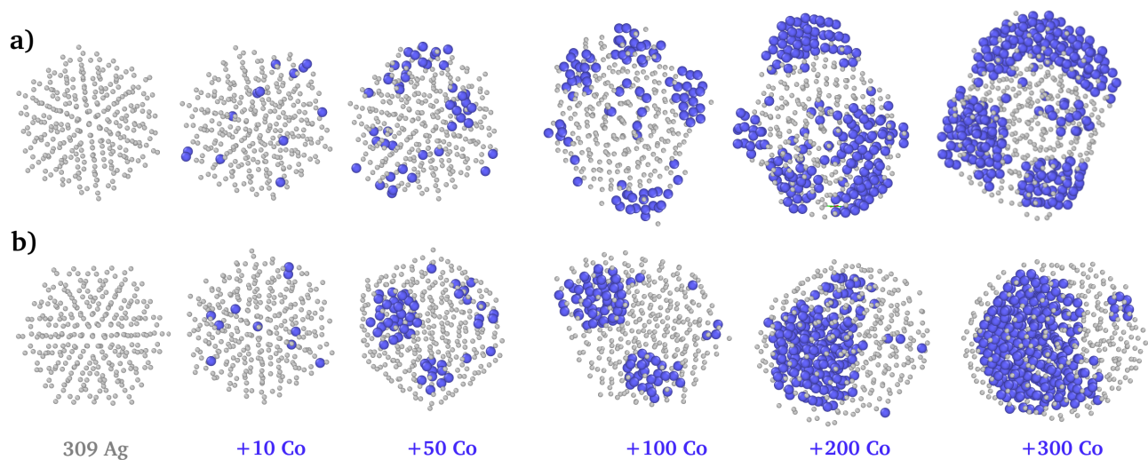
Fig. 5 Snapshots of the growth of Co on an initial Ag nanoparticle( Ih_{Ag309} ) at 300 K (a) and 600 K (b). The snapshots are taken at different stages of growth, of up to 50% Ag atom content. Co and Ag atoms are represented as blue and gray spheres, respectively.
