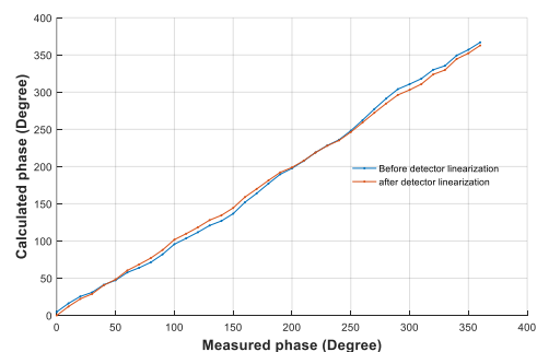
Figure 3 The calculated phases as a function of the measured phases with and without the detector linearization.
