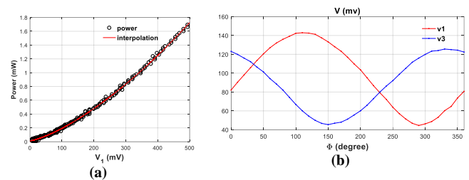
Figure 2 (a) Power in the detector 1 as a function of the voltage; (b) Detected voltage as a function of the phase
