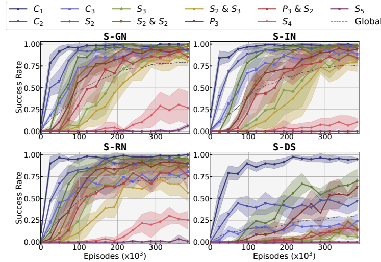
Figure 5: Local SR for each class across training episodes with continuous goals. Mean \pm standard deviations are computed over 5 seeds.
