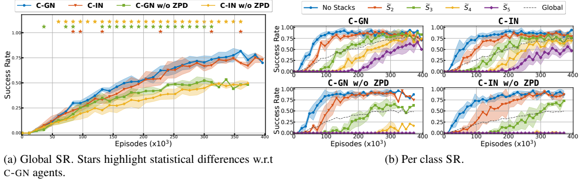
Figure 10: Performance metrics for C-GN, C-IN and their ablations where non-trivial scene reset is removed. Mean \pm standard deviations are computed over 5 seeds.
