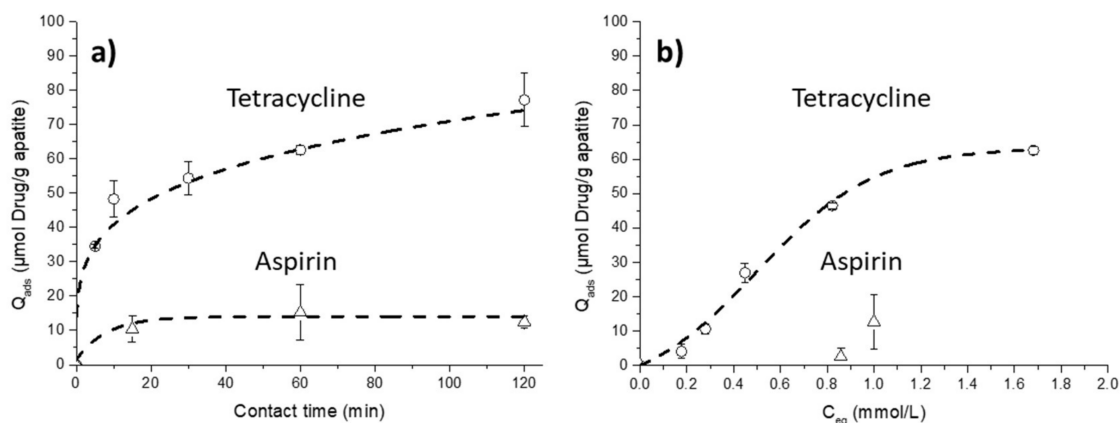
Figure 3. Drug adsorption on biomimetic apatite powder: (a) adsorption kinetics at pH = 7.4, room temperature and (b) adsorption isotherms at pH = 7.4, room temperature for 1 h; two drug adsorptions are performed with tetracycline (o) and aspirin ( \Delta ) using experimental protocol 1.
