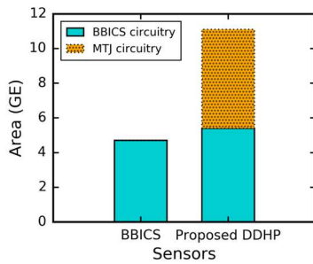
Figure 9: Area overhead represented in Gate Equivalents (GE) of the proposed DDHP architecture compared to a BBICS structure.
