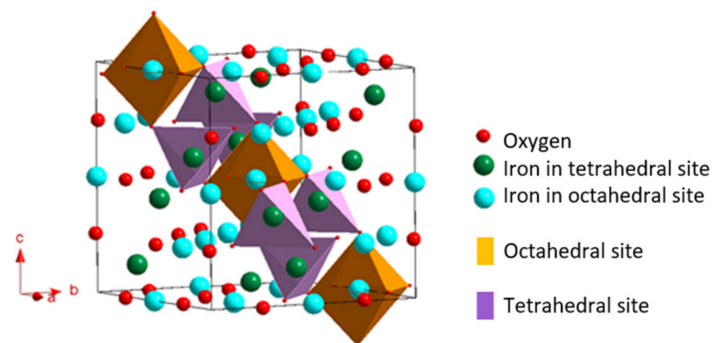
Figure 1. Representation of mesh of the crystallographic structure of magnetite. The octahedra and tetrahedra materialize on one of the planes (111) of the mesh.
