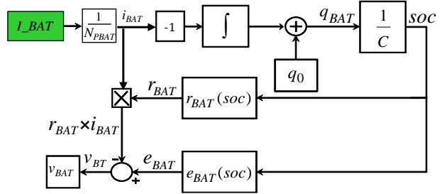
Fig. 6.b. Battery cell quasi-static electrical model
