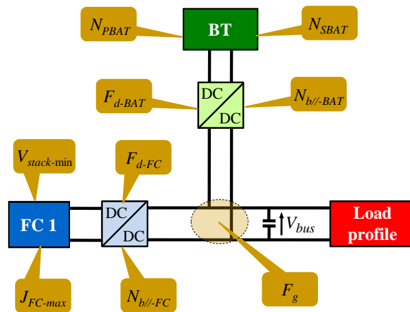
Fig. 14. The illustration of design variables
