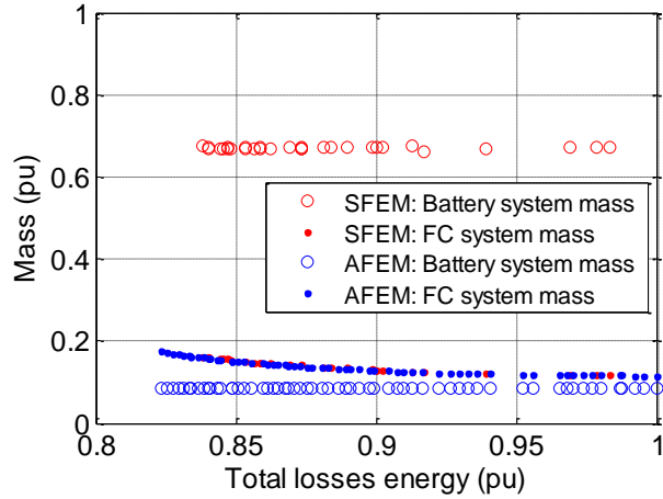
Fig. 16. The system mass distribution between the battery system (battery converter + battery) and the FC system (FC stack + FC converter + FC auxiliaries + H 2 tank)
