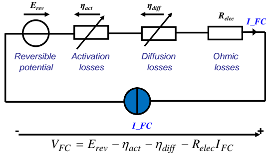
Fig. 6.a. Fuel cell quasi-static electrical model
