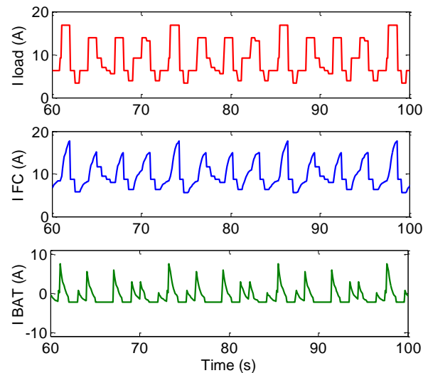
Fig. 7.b Simulation of the mission profile with Asymmetric Frequency Energy Management
