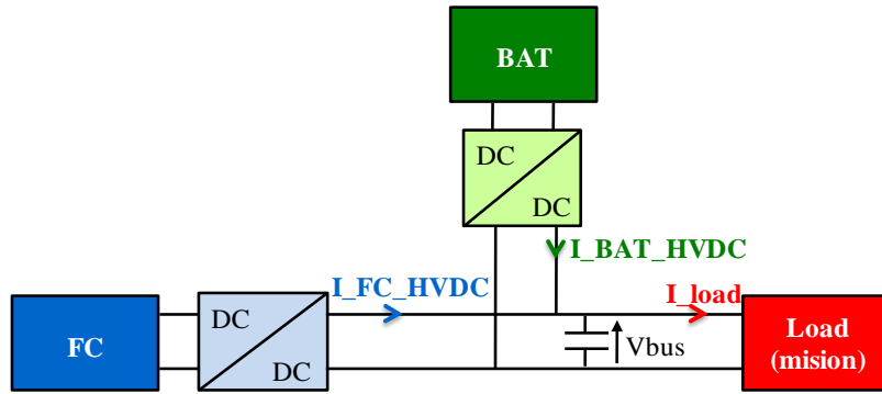
Fig. 8. The architecture of the experimental test bench
