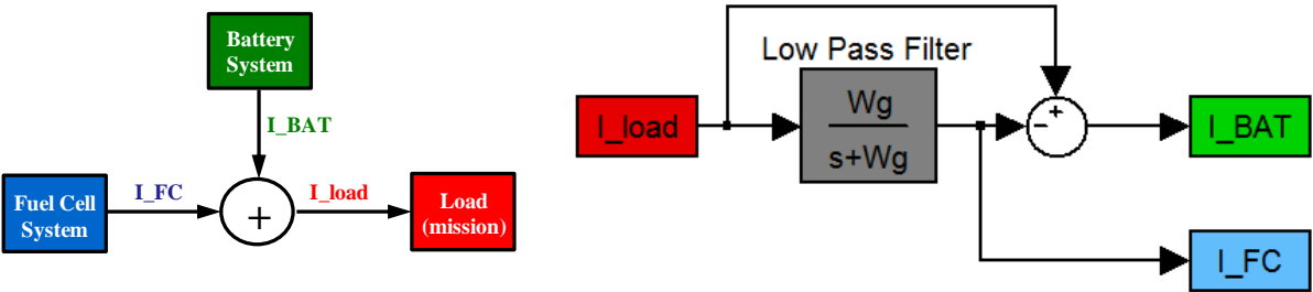
Fig. 2. Principle of Symmetric Frequency Energy Management
