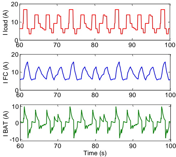
Fig. 7.a. Simulation of the mission profile with Symmetric Frequency Energy Management
