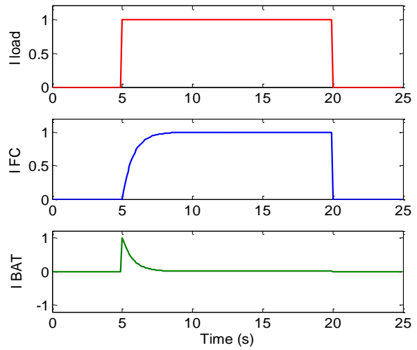
Fig. 3.b. Illustration of Asymmetric Frequency Energy Management
