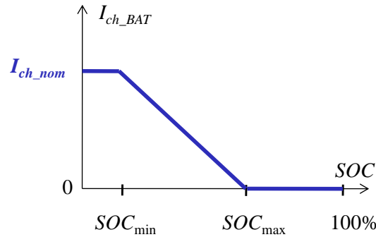
Fig. 4. The principle of the battery recharging loop
