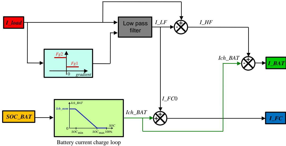
Fig. 5. Principle of the Asymmetric Frequency Energy Management
