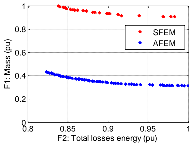
Fig. 15. Comparison of the two Pareto fronts obtained with symmetric and asymmetric energy management strategies
