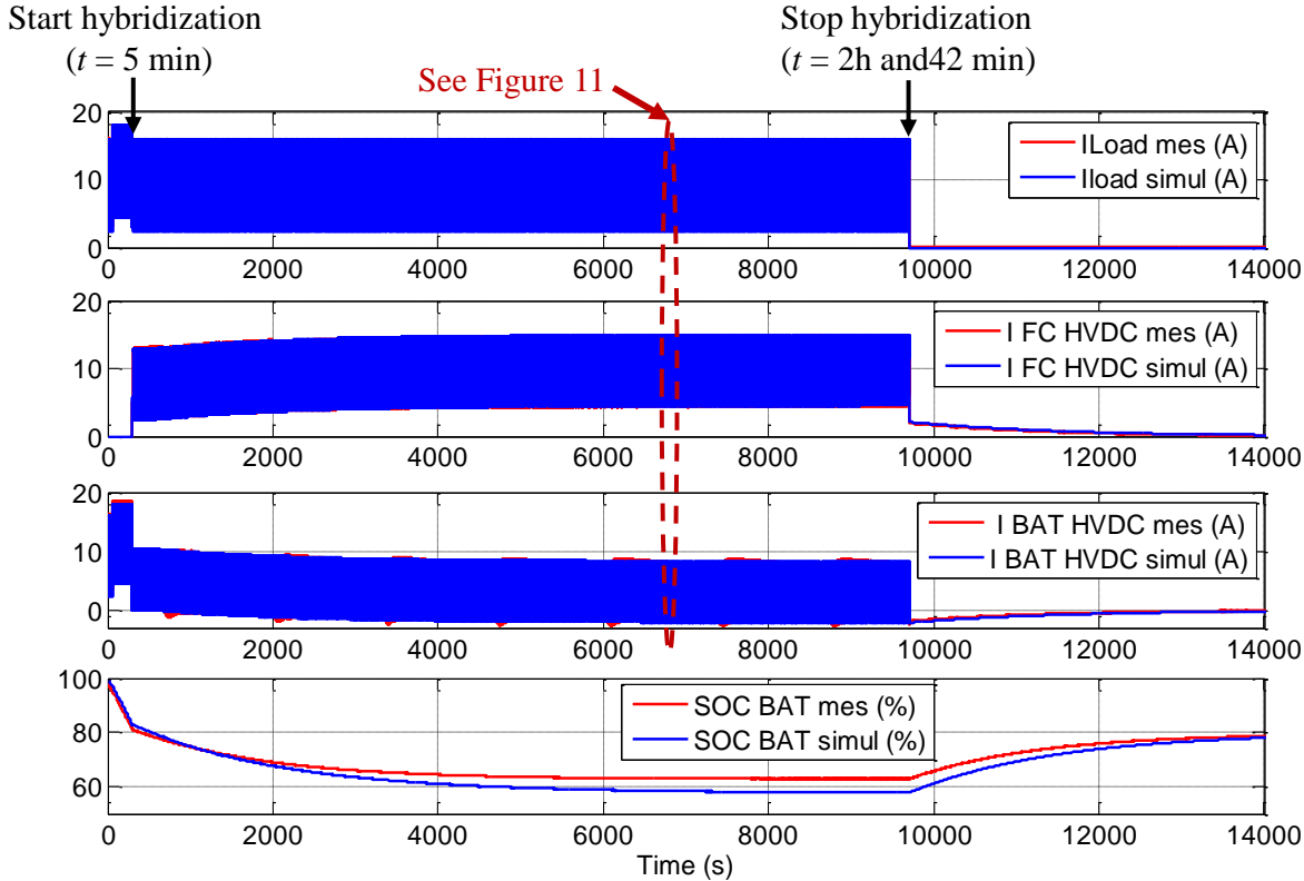
Fig. 10. The experimental and simulation results of Asymmetric Frequency Energy Management strategy
