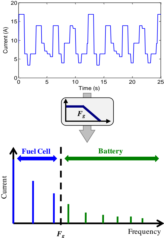
Fig. 1. Crossing between mission and source power sharing: (top graph: time chronogram of the mission profile, lower graph: frequency current sharing plan)
