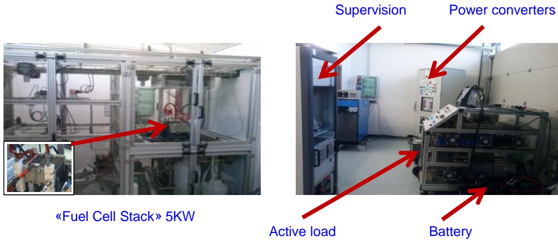
Fig. 9. The "FC-Li-ion Battery Hybridization" test bench on the « Hydrogen » platform of the LAPLACE laboratory
