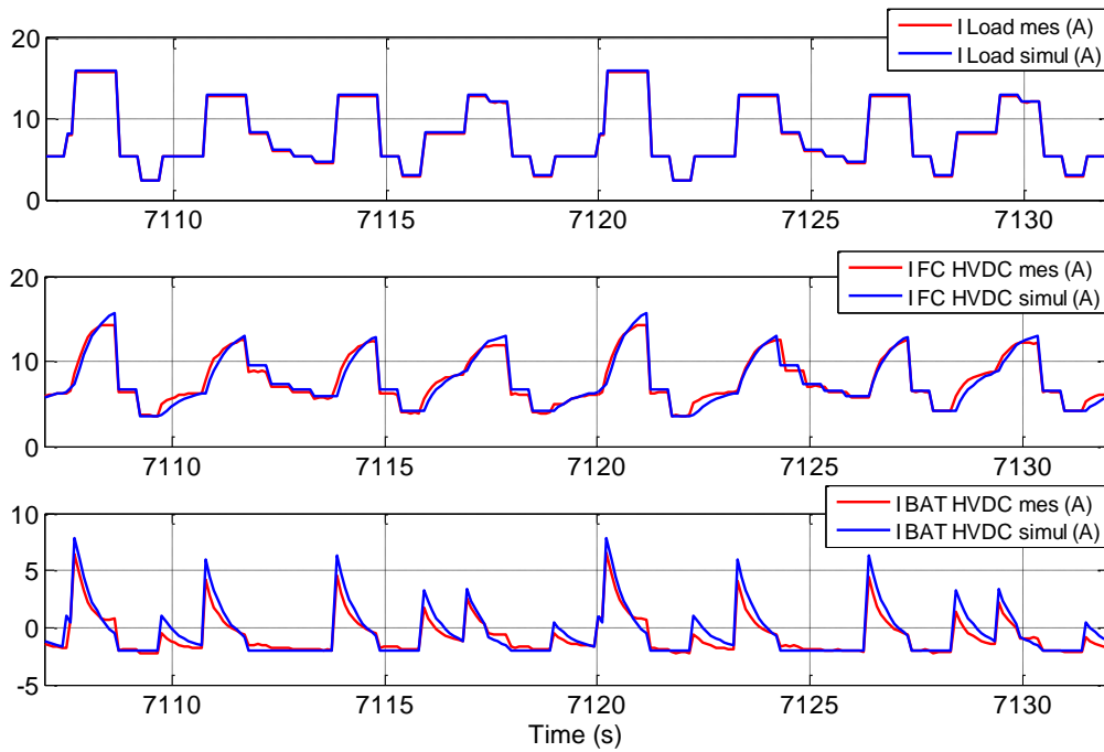
Fig. 11. Zoom of experimental and simulation results of Asymmetric Frequency Energy Management strategy
