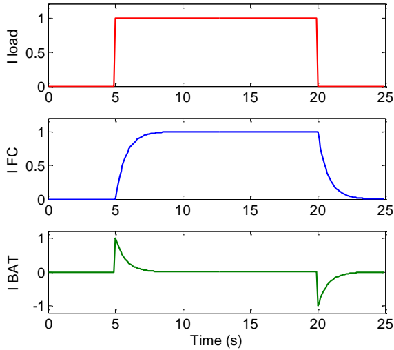
Fig. 3.a. Illustration of Symmetric Frequency Energy Management
