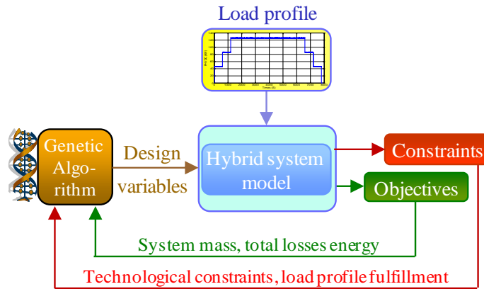
Fig. 13. Optimization process
