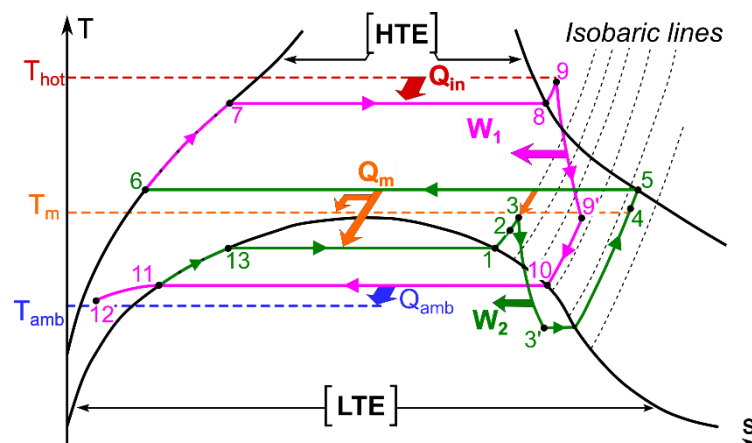
Fig. 5 – Combined charge and discharge power generation mode of the hybrid thermochemical cycle (single sorption cycle): thermodynamic path in the T–s diagram of ammonia (see Fig. 2 for caption details)
