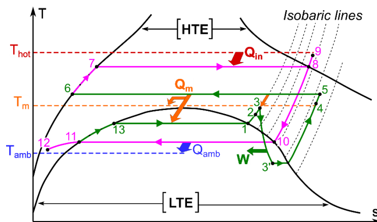
Fig. 4 – Discharge power generation mode of the hybrid thermochemical cycle (single sorption cycle): thermodynamic path in the T–s diagram of ammonia (see Fig. 2 for caption details)
