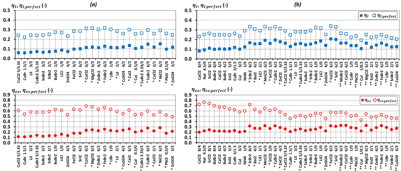
Fig. B1 – Discharge power generation mode: energy and exergy efficiencies of the cycle for selected salts
