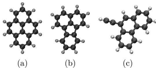
Figure 1: Molecular structures of the studied C 16 H 10 + isomers, optimized with the GAUSSIAN16 package at the B3LYP/6-31g(d,p) level of theory: (a) pyrene (Pyr + ), (b) fluoranthene (Flu + ), and (c) 9-ethynylphenanthrene (EtP + ).
