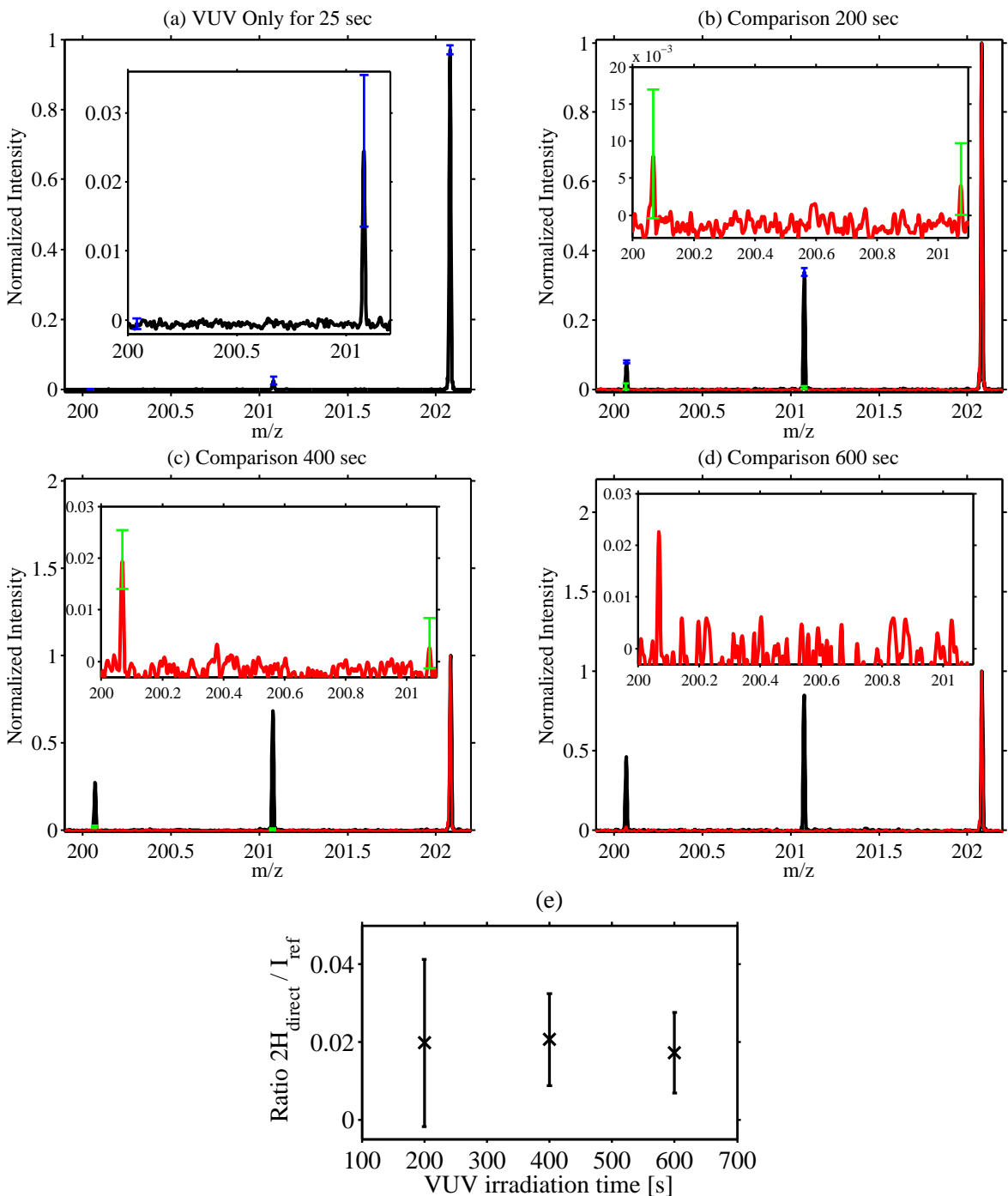
Figure S13: (a) Mass spectrum for a VUV irradiation time of 25 s. The insert is a zoom on the [Pyr-H] + and [Pyr-2H/H 2 ] + peaks. (b-d) Mass spectra for a VUV irradiation time of 200, 400, and 600 s respectively without [Pyr-H] + ejection (black curves) and with [Pyr-H] + ejection all 25 s (red curves). The inserts show a zoom on the [Pyr-H] + and [Pyr-2H/H 2 ] + peaks. (e) Ratio of the direct 2H/H 2 + loss peak to the total H and 2H/H 2 + production for the three VUV irradiation times, which leads to a value of 1.9 \pm 1.4\% .
