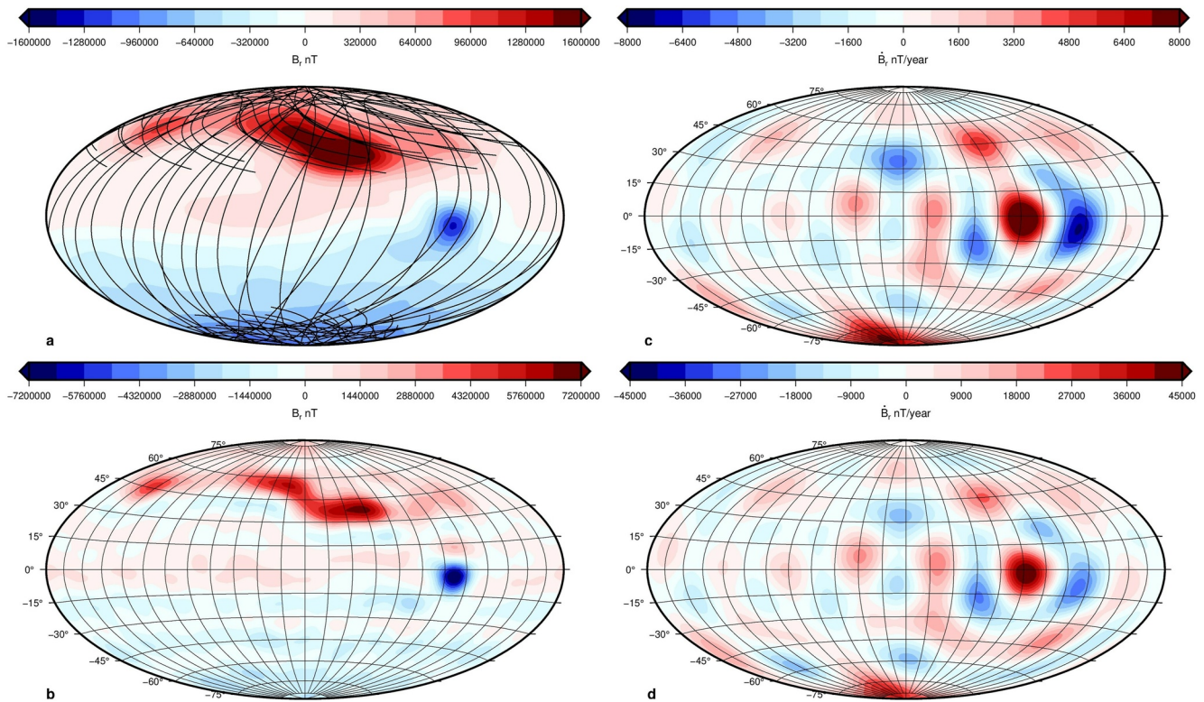
Figure 4. The (a, b) radial field and (c, d) its secular variation at (top) Jupiter's surface and (bottom) R_{Jf} . The maps are centered at 180^\circ longitude. The lines in (a) show the orbit paths of the used data set.
