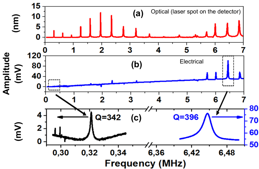
Figure 6: Optical and electrical response amplitude of a 440 \mu m long and 40 \mu m wide doubly clamped beam on a 700 nm thin buffer up to 7 MHz. (a) Optical Doppler vibrometry signal. (b) Electrical detection signal. (c) Zoom of the electrical signal for the first and 16 th flexural mode. The actuation voltage is V_{act} = -2 + 1 \cdot \cos(\omega t) V and the detector is DC biased at 900 mV.
