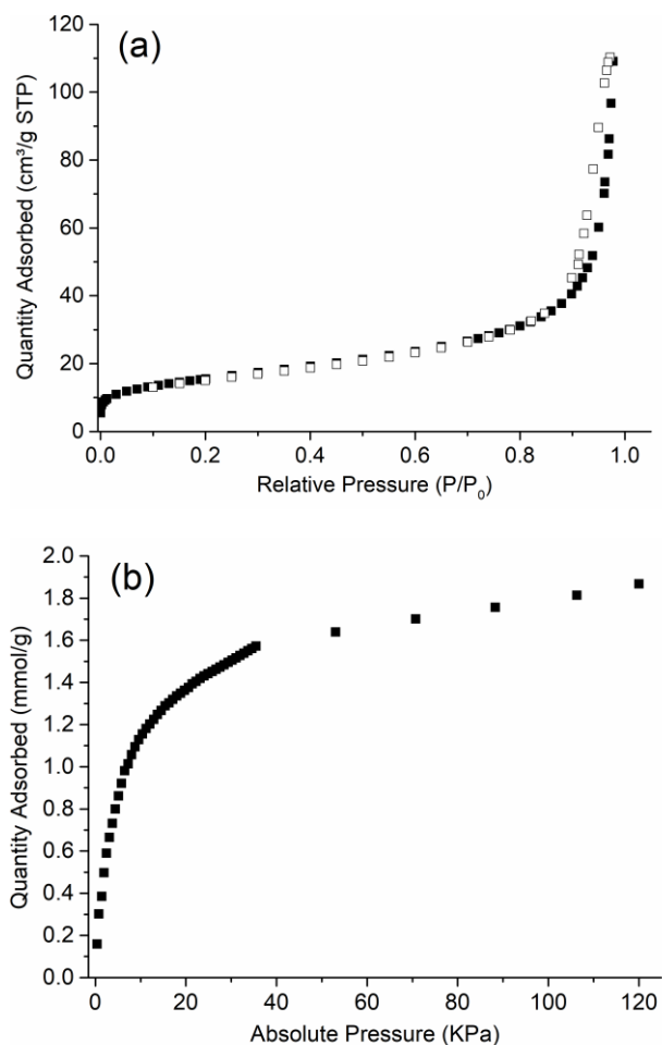
Figure 5. (a) \text{N}_2 adsorption (filled) and desorption (empty) isotherms measured at 77 K and (b) \text{CO}_2 adsorption isotherm measured at 273 K of the as-synthesized Na,Cs-RHO-2.0 nanozeolite.
