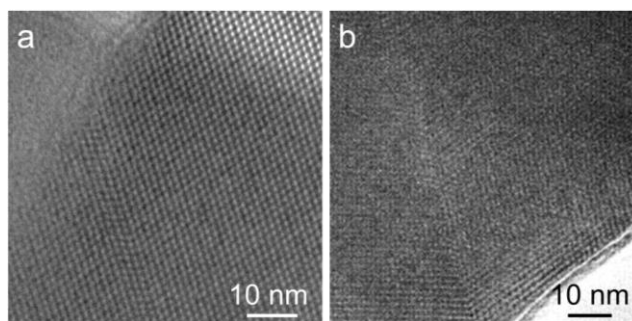
Figure 12 High-resolution TEM images showing the stacking fault (a) and typical twin interface (b) in zeolite Y.
