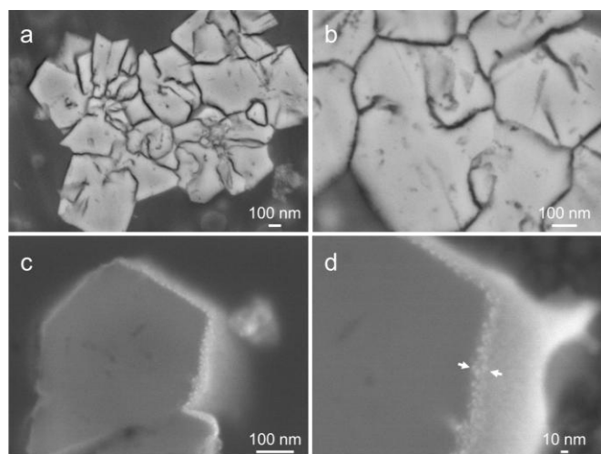
Figure 11 The ultra-high-resolution FE-SEM images of the cross-section of the Os-coated FY2 sample. In Figure 11c and d, Os was penetrated in mesopores. The presence of Os particles in the mesopores was indicated with white arrows.
