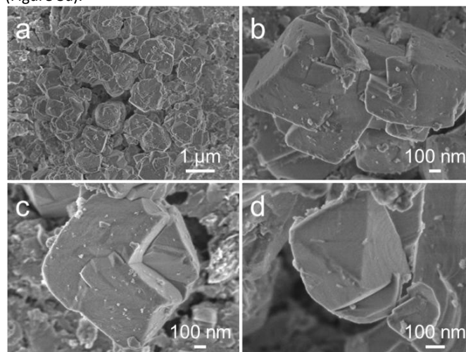
Figure 1 Low (a) and high (b) resolution SEM images of the parent zeolite.
