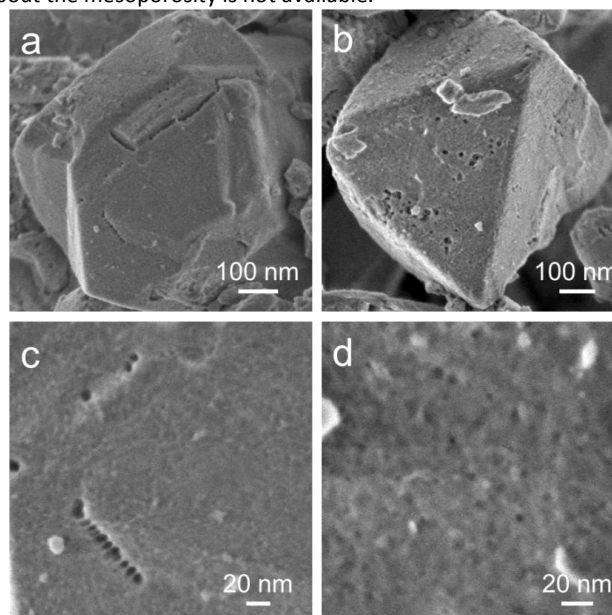
Figure 4 Low (a,b) and high (c,d) magnification SEM images of the FY1 sample.
