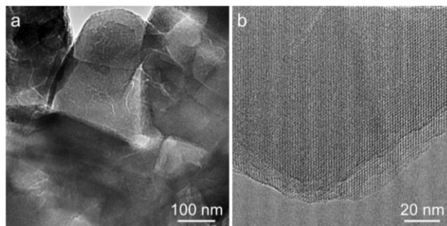
Figure 13 Low (a) and high-resolution (b) TEM images showing the intra-particle cracks induced by alkaline treatment.
