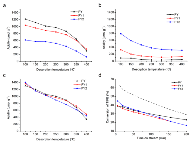
Figure 8 The Brønsted acidity (a), Lewis acidity (b), and summation of Brønsted and Lewis acidity (c) of the parent and \text{NH}_4\text{F} etched zeolite Y samples. (d) Dealkylation of 1,3,5 tri-isopropylbenzene (TIPB) on the parent and \text{NH}_4\text{F} etched zeolite Y samples (Reaction temperature = 453 K, W/F o = 0.022 kg h mol -1 , P = 0.1 MPa). Note: the dashed line shows the TIPB conversion on another mesoporous Y zeolite prepared by \text{NH}_4\text{F} etching of the same parent sample. 15 It is used as a reference sample here.
