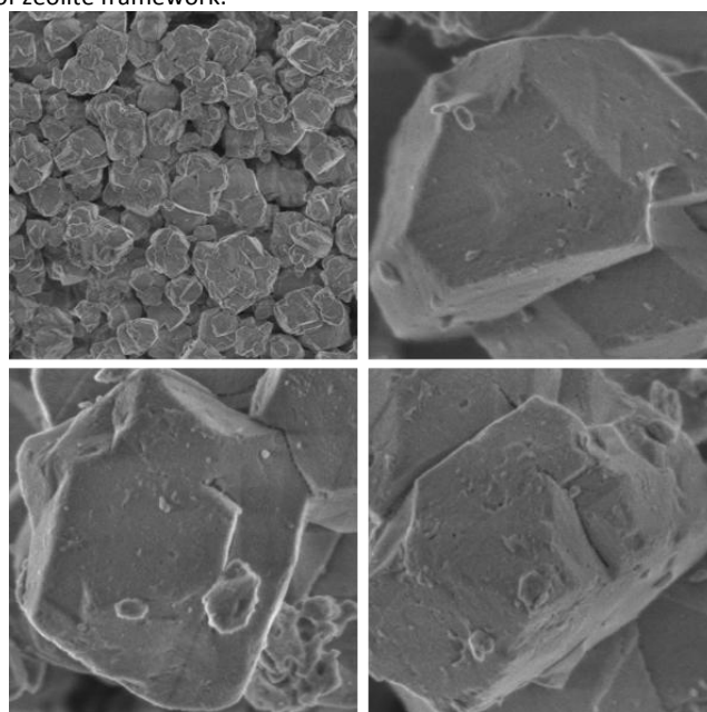
Figure 6 The SEM images of the zeolite Y sample after fluoride etching for 5 min in 25 wt% aqueous \text{NH}_4\text{F} solution.
