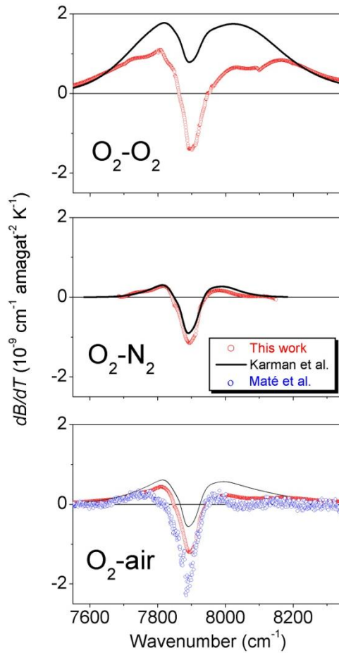
326 Figure 7. Comparison of the temperature dependence of the B_{O_2-O_2}(v_i) (upper panel), B_{O_2-N_2}(v_i) 327 (middle panel) and B_{O_2-air}(v_i) (lower panel) binary coefficients derived from CRDS measurements 328 (This work), FTS measurements (Maté et al., 1999) and theoretical calculations (Karman et al., 2018).
