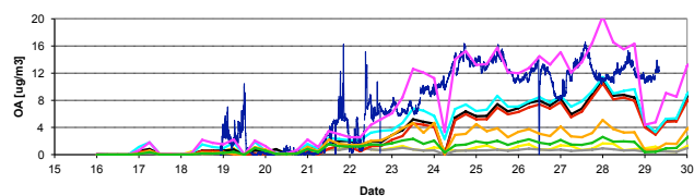
Fig. 4. AMS-measured (dark blue line) and modelled near-surface SOA mass concentration during June 2010 at Puy-de-Dôme, France. Grey line: according to Antila et al. (2010); yellow line: more VOC precursor gases; green line: SOG transport and removal; orange line: SOG transport and removal plus biogenic emissions \times 5 ; red line: 1. aging SOG – 1 % aging; black line: 2. aging SOG – 1 % aging, light blue line: 2. aging SOG – 10 % aging; magenta line: 2. aging SOG – 10 % aging plus biogenic emissions \times 5 . See the text for more explanation.
