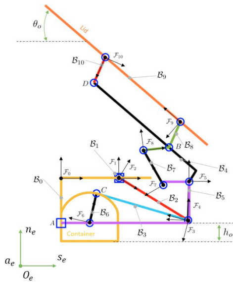
Fig. 4. The tree-like structure of the hinge.
