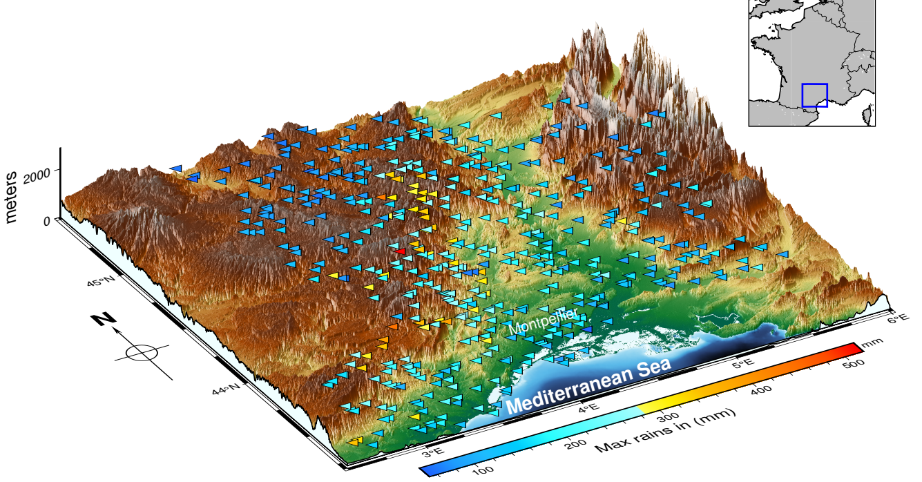
Figure 1: Historical (1958-2000) daily rainfall maxima in millimeters per station in the Cévennes-Vivarais region of France.
