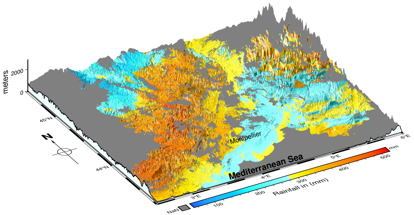
Figure 6: Estimation at a finer scale by the CENN quantile estimator at order 1 - \alpha_n = 1 - 1/n_o . The gray region is corresponds to Not a Number (NaN) results obtained when condition (38) is not satisfied.
