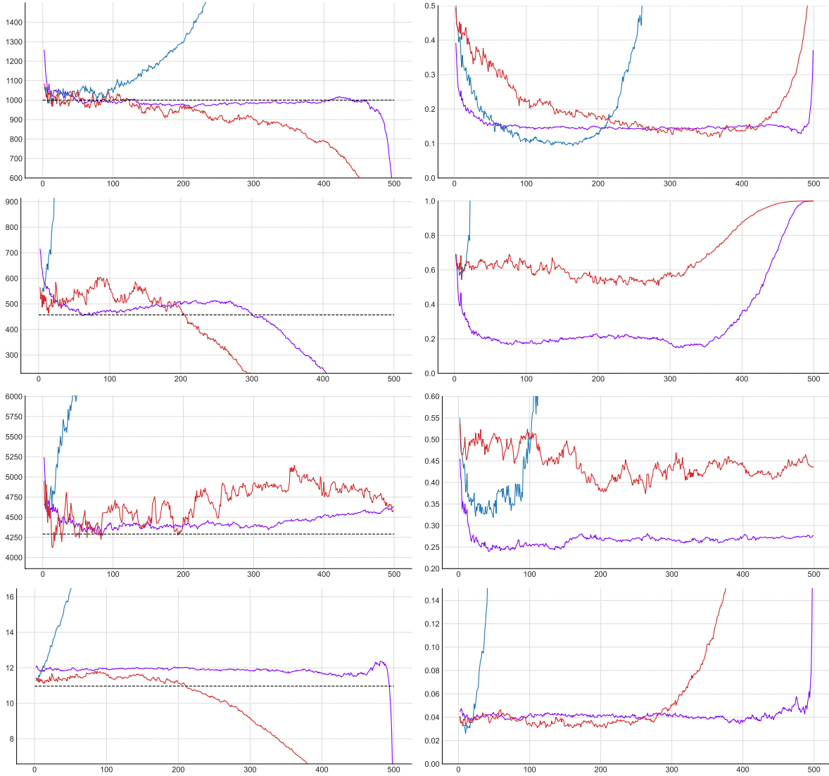
Figure 3: Illustration on simulated data sets of size n = 500 from a Burr distribution with \gamma = 1 and \rho \in \{-2, -1/4\} , a NHW distribution with \gamma = 1 and \rho = -1/8 , and a GPD distribution with \gamma = 1/8 (from top to bottom). Median of the estimators (left panel) of the extreme quantile (black dashed line) at level 1 - \alpha_n = 1 - 1/(2n) and RMedSE (right panel), as functions of k \in \{2, \dots, n - 1\} , computed on R = 500 replications, associated with W (blue), RW (red) and NN (purple) estimators.
