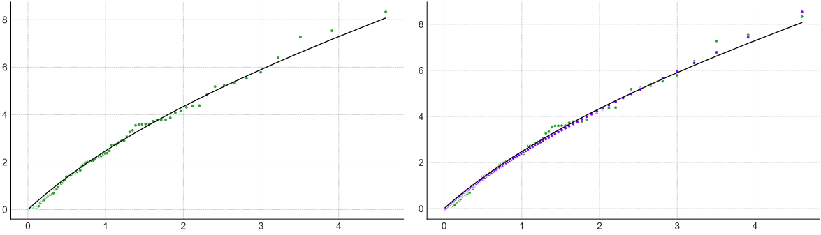
Figure 2: Log-spacing function associated with a Burr distribution ( \gamma = 1, \rho = -1/4 ). Black curve: theoretical function x_1 \mapsto f(x_1, \log(n/k)) , green dots: empirical pointwise estimation (\log(k/i), \log X_{n-i+1,n} - \log X_{n-k+1,n}) , purple dots: NN estimation \tilde{f}_{\hat{\phi}}^{\text{NN}J}(\log(k/i), \log(n/k)) with i = 1, \dots, k-1, k = 100 and n = 500 .
