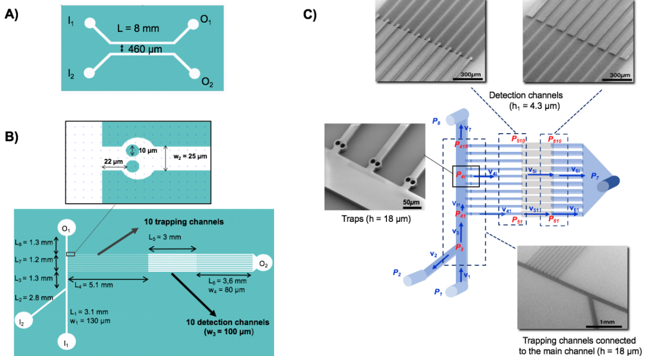
FIGURE 2 Microfluidic devices. (A) 2D-Clewin drawing of the virometry chip. The two identical microchannels have an inlet (I) and an outlet (O). (B) 2D-Clewin drawing of the viro-fluidic chip. Ten individual trapping channels were disposed upstream of 10 detection channels and perpendicular to the main channel connecting the inlet ( I_1 ) and outlet ( O_1 ). Cells were perfused in I_2 and the viral particles exited through O_2 . Lengths ( L_i ) and widths ( W_i ) of each microchannel section are indicated. The upper inset gives an enlargement of a trap that was composed of two cylindrical pillars ( d = 10 \mu\text{m} ) separated by 4 \mu\text{m} . (C) Images of scanning electron microscopy of the master mold (grey rectangles) of the viro-fluidic chip show the photoresist (SU8) deposited on a Si wafer. The central drawing shows the trapping channels ( h : 18 \mu\text{m} ) in blue and the detection channels ( h : 4.3 \mu\text{m} ) in grey. The external applied pressures and average flow speeds in each channel section are shown in blue and the internal pressures in red.
