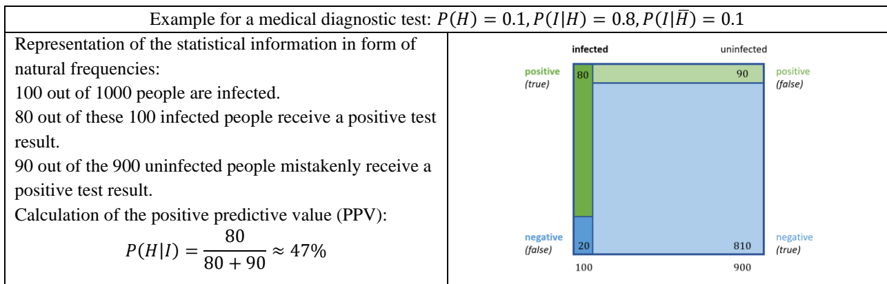
Figure 1: Example for the two beneficial strategies representing the statistical information with natural frequencies and depicting the situation in a visualization, here the unit square
