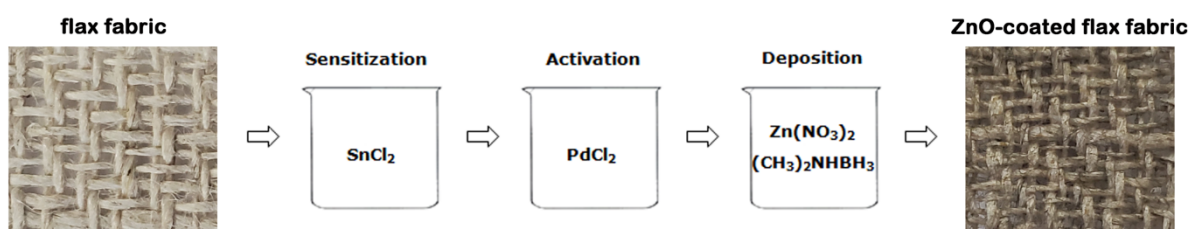
Figure 1. Schematic representation of the steps involved in the functionalization of the flax fabrics by ZnO electroless deposition.
