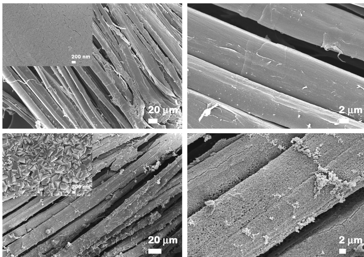
Figure 3. FESEM images at different magnifications of flax fibers ( top ) and ZnO-coated flax fibers ( bottom ) as fabrics.
