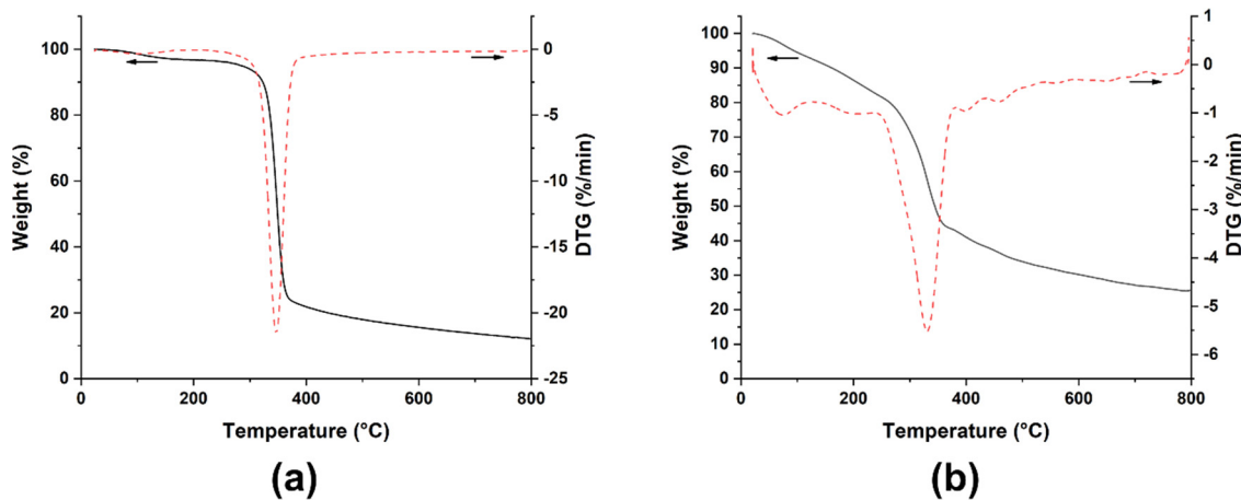
Figure 7. TGA (black solid curves) and dTG (red dot curves) thermograms of (a) neat flax yarns and (b) ZnO-coated flax yarns (arrows indicate the corresponding Y axis).
