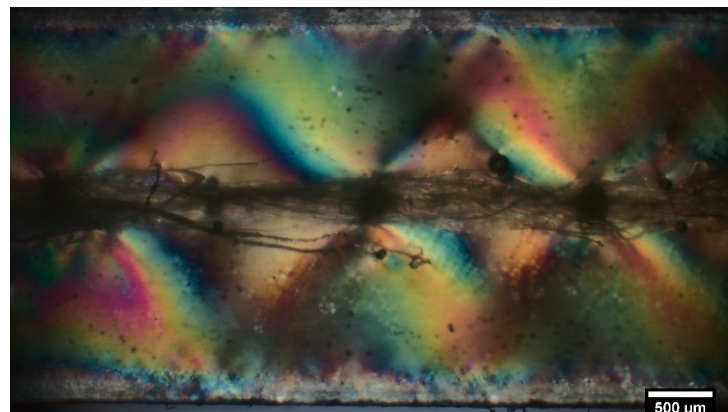
Figure 9. Birefringence effects of fragmented ZnO-coated flax yarns.
