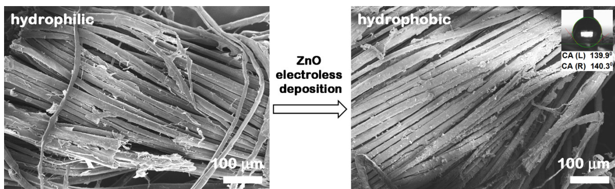
Figure 5. FESEM images of flax and ZnO-coated flax fibers as fabrics. In the inset is shown the optical photograph of the water droplet shape on the hydrophobic surface of ZnO-coated flax fabrics and the water contact angles for the corresponding sample.
