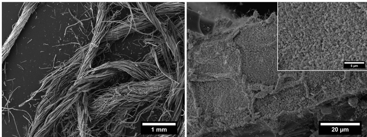
Figure 8. FESEM images at different magnifications of ZnO-coated flax yarns after the thermogravimetric test.
