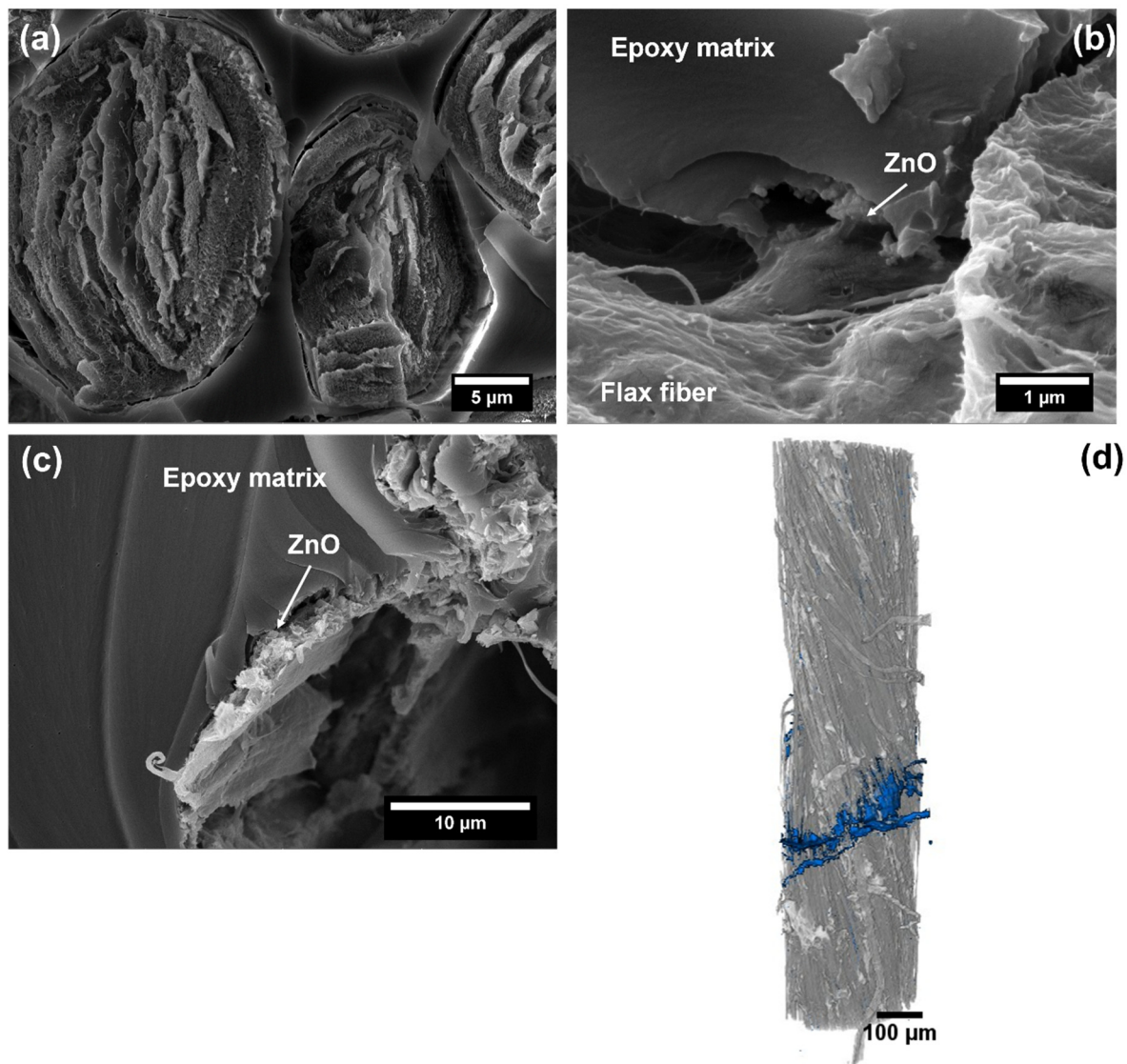
Figure 10. (a–c) FESEM images, at different magnifications, detailing the fracture morphology of a single ZnO-coated flax yarn composite after the single yarn fragmentation test and (d) volumetric reconstruction from micro-CT scans of ZnO-coated flax yarn (dark grey) and the fracture zone (blue).
