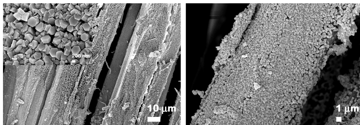
Figure 4. FESEM images at different magnifications of ZnO-coated flax fibers as yarns.
