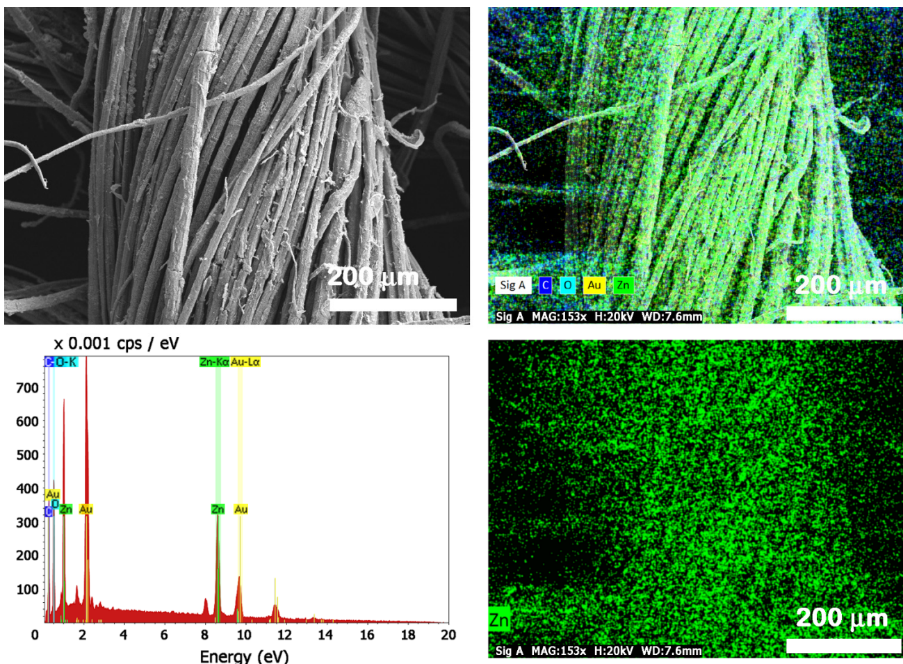
Figure 6. FESEM image, EDX mapping and EDX spectrum of ZnO-coated flax fabrics and the EDX mapping only for Zn element.
