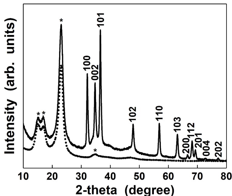
Figure 2. XRD patterns of flax (dotted curve) and ZnO-coated flax fibers (solid curve) as fabrics. * Peaks attributed only to flax fibers.
