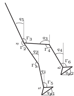
Figure 2: Generalized coordinates, and inter-link torques.
