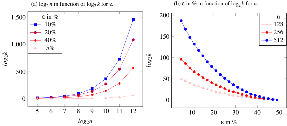
Figure 1: Link between k and n or \epsilon .
