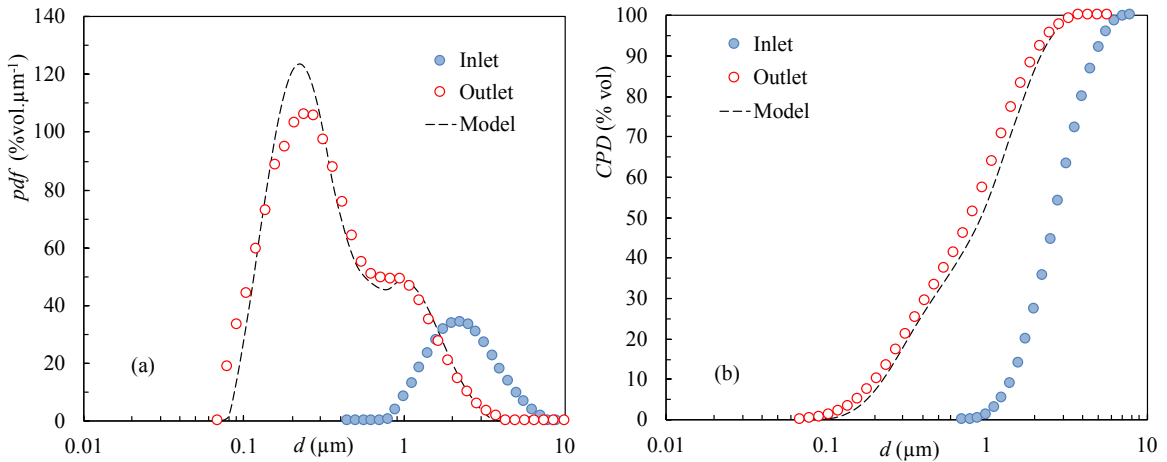
Figure 10: Size distribution of milk fat globules in the pilot scale HPH at 120 bars and 80°C. Comparison between model (dashed line) and experiments (symbols). (a) pdf (b) CPD ( K_1=2.22 , K_2=10 , \Phi_2=36\% )
