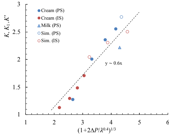
Figure 12: Fragmentation constant as a function of (1 + 2\Delta P/\lambda^{0.4})^{1/3} for all systems in both HPH geometries. Closed round symbols: experimental data for cream \lambda=3.69 ( \mu_e=2.9 \times 10^{-3} ). Open round symbols: simulation data with \lambda=9.25 ( \mu_e=1.16 \times 10^{-3} ). Triangle symbol: milk with \lambda=1.69 ( \mu_e=0.63 \times 10^{-3} ). Blue color: pilot scale (PS). Red color: industrial scale (IS)
