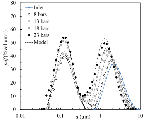
Figure 9: pdfs of cream globule size in the industrial scale HPH . Comparison between model (dashed line) and experiments (symbols) K_1=(1.12, 1.29, 1.48 \text{ and } 1.70) and \Phi_2=(6.5, 7.1, 8.6 \text{ and } 8.7 \text{ \%}) respectively for \Delta P=(8, 13, 18 \text{ and } 23 \text{ bars}) . K_2=17.8 for all cases
