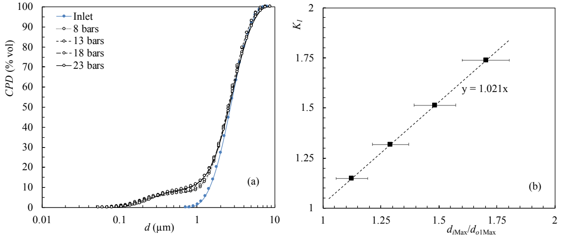
Figure 7: (a) Same curves as in Fig.6(b) for industrial HPH after multiplying the abscissas by a factor K_1 ( K_1 = 1.12, 1.29, 1.48 and 1.70 ) for ( \Delta P = 8, 13, 18 and 23 bars), respectively. (b) K_1 as a function of inlet-to-outlet maximum volume fraction diameter ratio. Error bars correspond to the width of a size class divided by the class size (i.e. \pm 6\% ). The uncertainty on K_1 is smaller than the symbol size on this graph.
