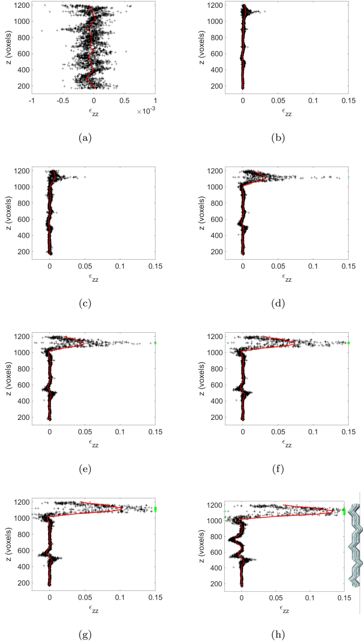
Figure 19: Vertical strain in the fiber \epsilon_{zz} as a function of vertical position of element center of gravity z for scans 01 (a), 02 (b), 03 (c), 04 (d), 05 (e), 06 (f), 07 (g) and 08 (h) of sample P1. The red line depicts the k -point mean values (with k = 100 vx). Data whose level does not lie within the selected range are shown with a saturated value in green.
