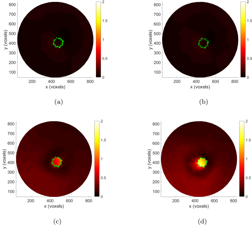
Figure 9: Norm of the displacements \|\mathbf{U}\| (expressed in voxels) for sample P2. x - y sections of scan 01 for z = 650 vx (a) and z = 850 vx (b). x - y sections of scan 03 for z = 650 vx (c) and z = 850 vx (d). The nodes belonging to the interface are represented in green.
