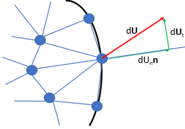
Figure 7: Decomposition of the displacement jump vector d\mathbf{U} into normal dU_n and tangential dU_t components
