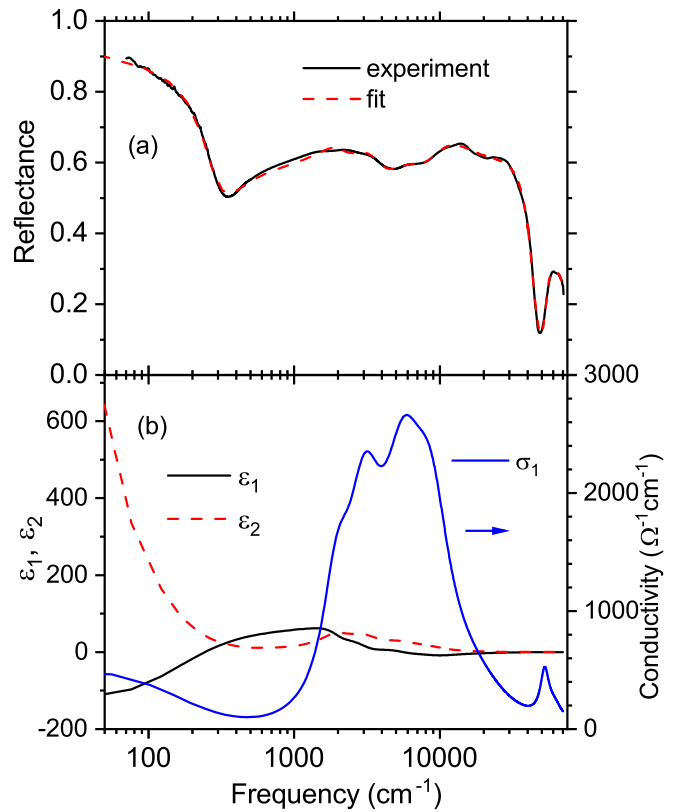
FIG. 4. (a) Room-temperature reflectance and its fit over the entire spectral range on a logarithmic scale. (b) Calculated complex dielectric function \hat{\epsilon} = \epsilon_1 + i\epsilon_2 and the real part of optical conductivity \sigma_1 = \nu\epsilon_2/60 , where \nu is in \text{cm}^{-1} and \sigma_1 is in \Omega^{-1} \text{ cm}^{-1} .
