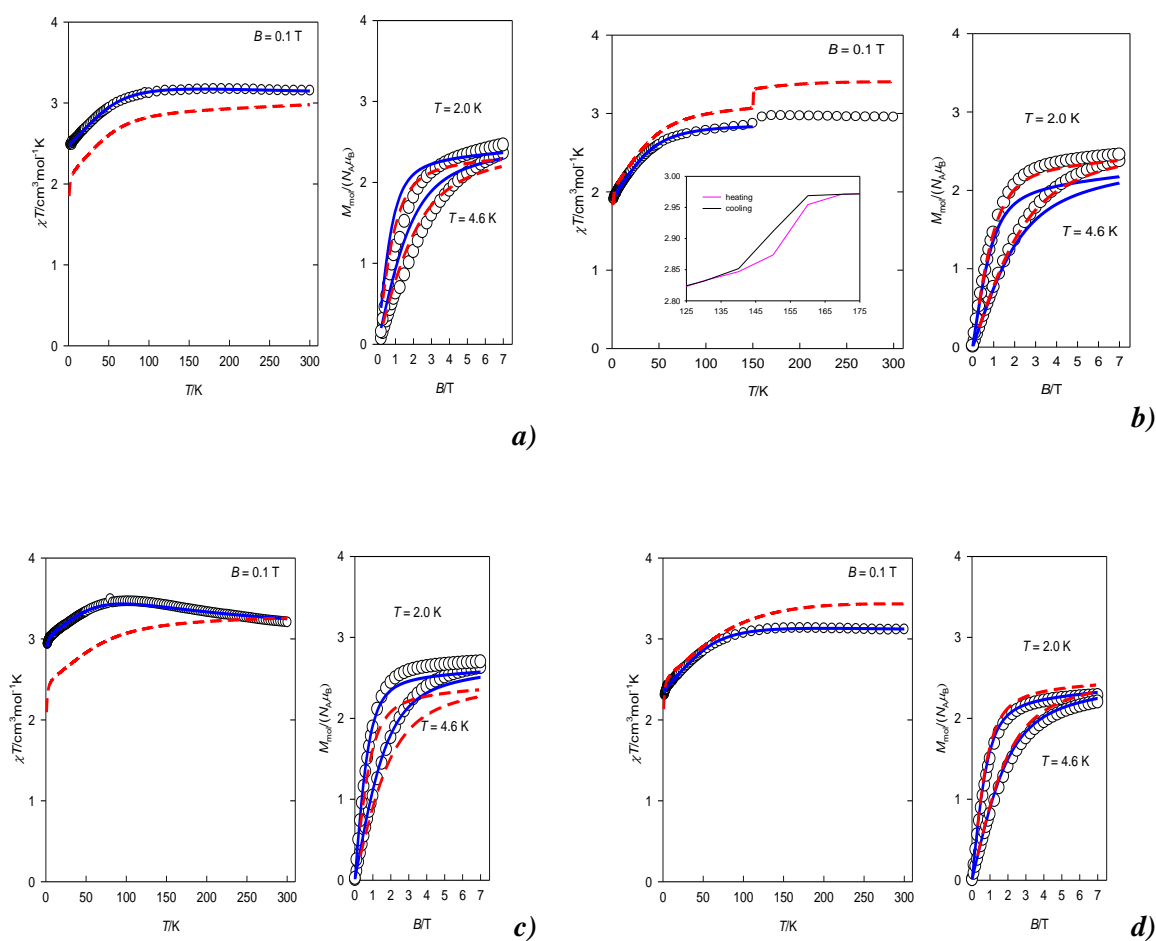
Figure 3 Magnetic functions analyzed by Spin Hamiltonian for a ) compound 1 ; b ) compound 2 ; c ) compound 3 and d ) compound 4 . Left: susceptibility-temperature product with respect to temperature, right: magnetization per center with respect to the magnetic field; empty circles: experiment, blue solid line: optimum fit, red dashed line: ab-initio prediction based on model molecules.
