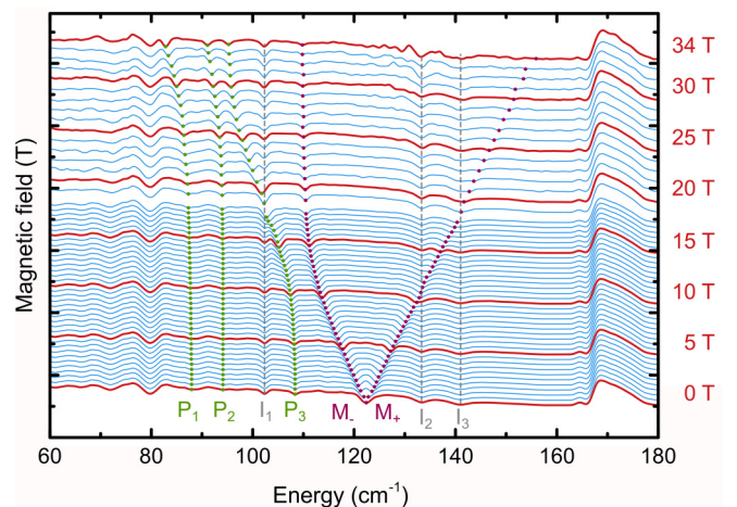
FIG. 2. Low-temperature ( T = 4.2 K) far-infrared transmission spectra for selected values of the magnetic field applied perpendicular to the layer planes, in the spectral region 60–180 \text{cm}^{-1} . Transmission minima denoted as P_i ( i = 1, \dots, 3 ) and M_+/M_- have their counterparts in resonances observed in Raman scattering spectra. I_i ( i = 1, \dots, 3 ) transitions are only visible in FIR transmission spectra. The pronounced minimum at \sim 80 \text{cm}^{-1} is due to absorption resonance in the polyethylene foil used in our experimental setup to filter the high-frequency radiation.
