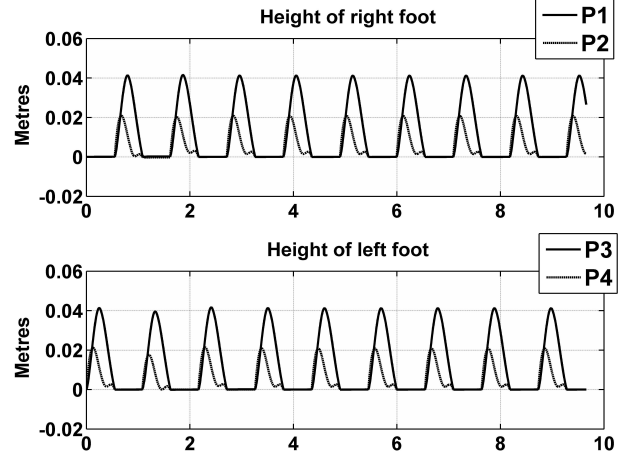
Fig. 2. Foot height in the walking gait with 0.5 s settling time
