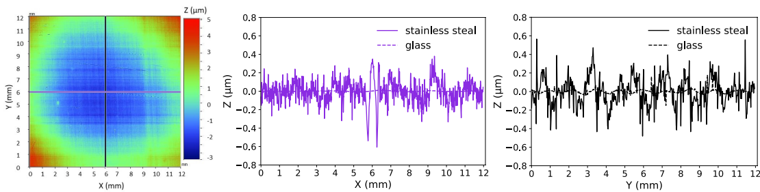
Figure 4. Profilometer stainless steel plate depth mapping, and depth profiles along X and Y for the lines drawn on the map.
