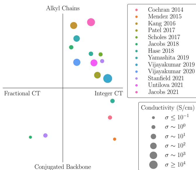
Fig. 2 Compilation of available experimental data for PBT TT and P3HT, relating the position of molecular dopants in the polymer lamellae (alkyl chains vs. conjugated backbone) to the nature of the host-dopant complexes (integer vs. fractional CT). The electrical conductivities of each sample is expressed through the size of the marker, see legend. The position of different points in each quadrant is arbitrary. We note that the large majority of doped polythiophenes feature integer CT, except for two systems corresponding to dopants inserted in the conjugated backbones. The systems with the largest conductivities are characterized by dopants inserted in the alkyl region and integer CT (upper-right quadrant).
