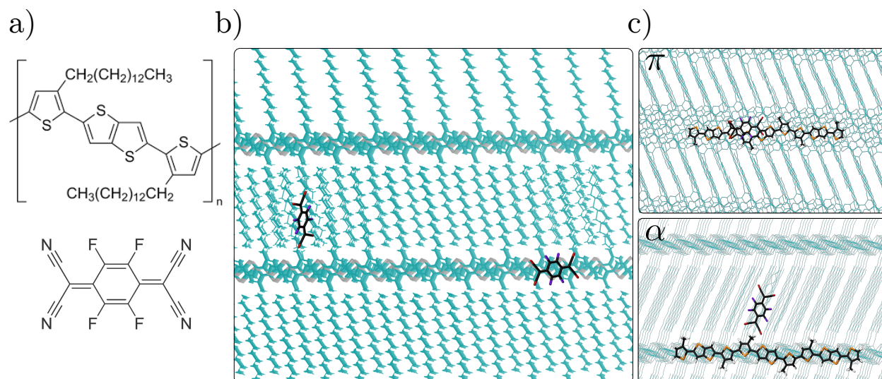
Fig. 1 (a) Chemical structures of the PBT TT polymer and F4TCNQ dopant investigated in this work. (b) Crystalline PBT TT lamella viewed from the top of stacked polymer-backbone chains, characterized by alternating conjugated and alkyl regions. The two F4TCNQ molecules illustrate the two positions of the dopant molecule considered in this work. (c) Rendering of the DFT/MM-optimized complexes with dopant in the conjugated region ( \pi structure, top) and in the alkyl chains ( \alpha structure, bottom) that have been employed in the calculations. The subsystems described at the quantum level (QM region of our QM/MM calculations) are shown in bold, the classical embedding environment (MM region) is drawn with thin lines.
