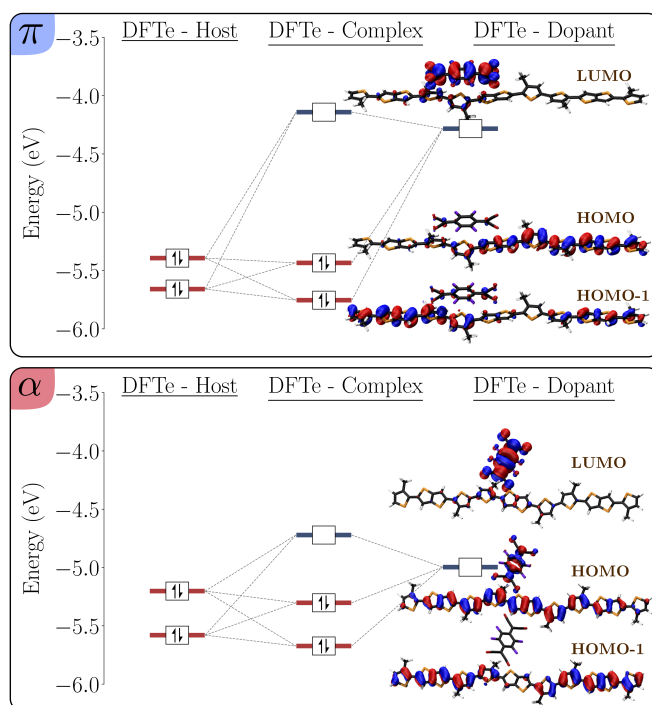
Fig. 5 Frontier energy levels diagram for the \pi (top) and the \alpha -BTTT-F4TCNQ complexes, as obtained from spin-restricted (RKS) DFT/MM calculations. Intermolecular orbital hybridization leads to an opening of the gap with respect to non-overlapping fragments (left- and right-most levels), and to a fractional CT ground-state in both systems ( Q_{\text{dop}} \approx -0.2 , see text).
