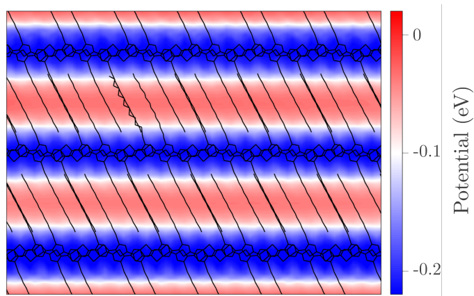
Fig. 4 Electrostatic potential map of the PBTTT crystal obtained from classical microelectrostatics calculations, illustrating the remarkably difference in potential experienced by dopants placed in the region of the conjugated backbone with respect to the alkyl side chains. The local potential has been obtained using a 5 Å-radius spherical probe and averaged over the c crystal axis, perpendicular to the figure plane. The calculation considers periodic boundary conditions in 2D in the ab crystal plane.
