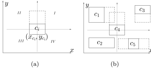
Fig. 13 Relative position (a) Definition, (b) Representation.
