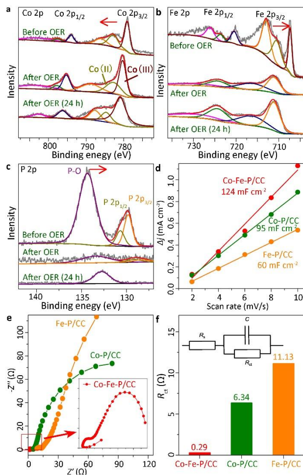
Figure 5. (a-c) High-resolution XPS spectra of (a) Co 2p, (b) Fe 2p and (c) P 2p of Co-Fe-P/CC before and after OER test. (d) Simulated plots of C_{dl} , (e) EIS plots, and (f)
