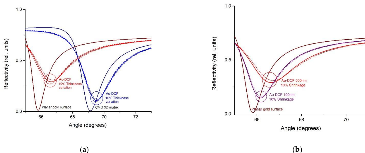
Figure 3. (a) Theoretical SPR curves on planar gold surface (dark red) and CMD-coated gold surface (dark blue); the addition of Au-DCF shifts the SPR curve minimum to higher angles: coated planar gold surface (continuous red line), coated CMD (continuous blue line); dotted and dashed lines show the effect of the \pm 10\% variation of the thickness of dynamer; (b) Theoretical SPR curves on planar gold surface (dark red) covered with a layer of 100 nm Au-DCF (purple) and 500 nm Au-DCF (red). The effect of 10% contraction of the Au-DCF is shown in dotted lines.
