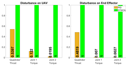
Fig. 11: End Effector normalize force and torque variation.
