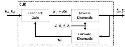
Fig. 4: Closed-loop inverse kinematic block diagram.
