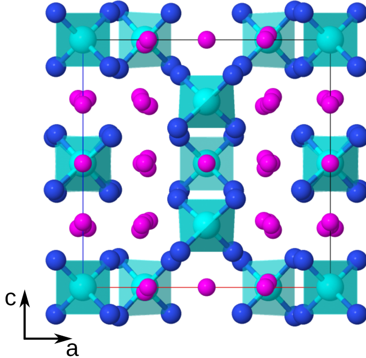
Figure 2: View of the LMN unit cell in the projection on the ac crystallographic plane. Color legend: cyan - manganese, blue - nitrogen, pink - lithium.
