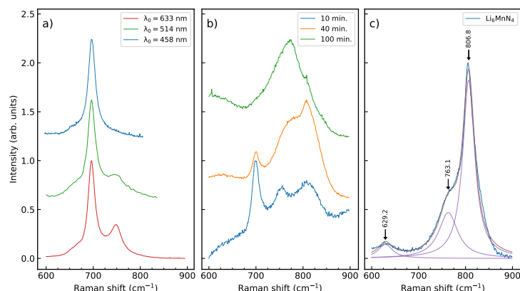
Figure 8: a) – Raman spectra of LMN powder sample in the airtight cell, measured with different wavelengths of the incident radiation \lambda_0 . b) – Raman spectra of LMN powder sample obtained 10 min., 40 min., and 100 min. after opening the airtight cell, measured with \lambda_0=633 nm. c) – Raman spectrum of electrochemically oxidized \text{Li}_6\text{MnN}_4 electrode sample in the airtight cell, measured with \lambda_0=633 nm.
