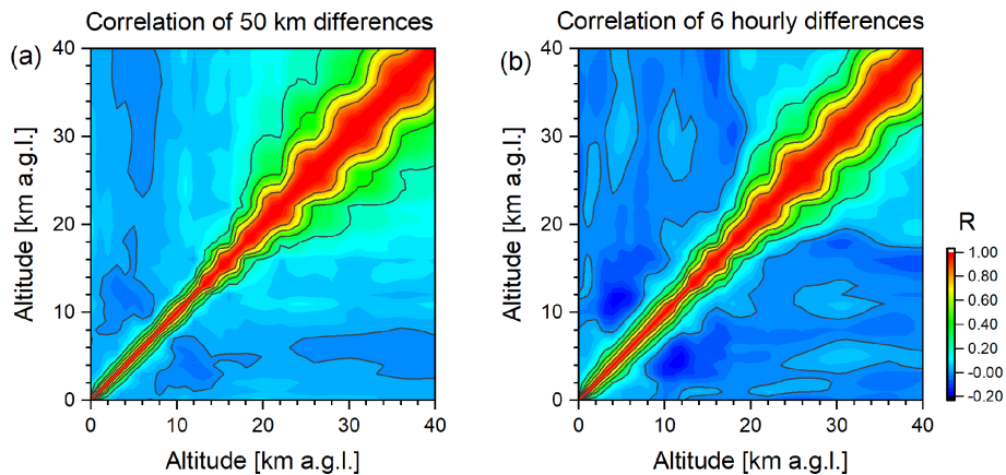
Figure E2. Characteristics of the vertical dependencies covered by the matrices S_{\Delta_{dl}}^l . Shown are the vertical correlation matrices for the difference between the reference CH 4 profile (location 49.1° N, 8.4° E, corresponding to the location of Karlsruhe) and profiles dislocated with respect to the reference: (a) horizontal dislocation of 50 km and (b) temporal dislocation of 6 h.
