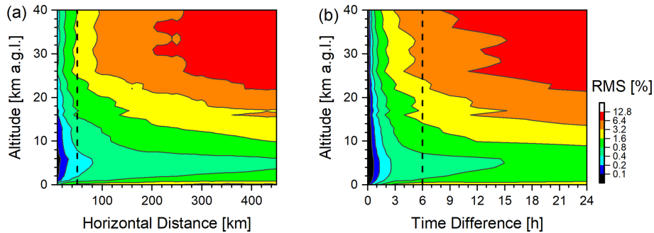
Figure E1. Square root values of the diagonal entries of different dislocation covariance matrices ( S_{\Delta_{dl}}^l ). These values are the root-mean-square (rms) of the difference between the reference methane profile (CAM5 forecast for location 49.1° N, 8.4° E, corresponding to the location of Karlsruhe) and other forecasted profiles dislocated with respect to the reference: (a) horizontal dislocations and (b) temporal dislocations. The dashed black lines indicate the collocation threshold values used for valid combinations of IASI and TROPOMI.
