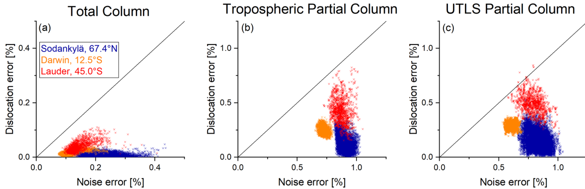
Figure E5. Comparison of the dislocation error (due to the CH 4 dislocation uncertainty) and the noise error (an example of the typical temporal dependencies of the noise error is shown in Fig. 6). The comparison is depicted for a northern high-latitude location (Sodankylä; violet crosses), a tropical location (Darwin; orange crosses), and a southern middle latitudinal location (Lauder; red crosses). (a) Total-column product, (b) tropospheric partial-column product, and (c) UTLS partial-column product.
